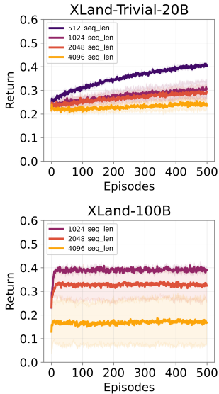
Figure 8: AD performance on our datasets for different sequence lengths. Both datasets lead to the emergence of in-context ability. We report the average return on 1024 unseen tasks across 3 seeds.
