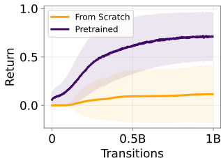
Figure 3: Single-task evaluation curves on 36 hard tasks for policies trained from scratch or fine-tuned from multi-task pretrained checkpoints. See Appendix D for curves on tasks of all difficulty.
