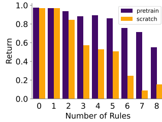
Figure 10: Final return by number of rules on 256 tasks for policies trained from scratch or fine-tuned from multi-tasks pre-trained checkpoints.
