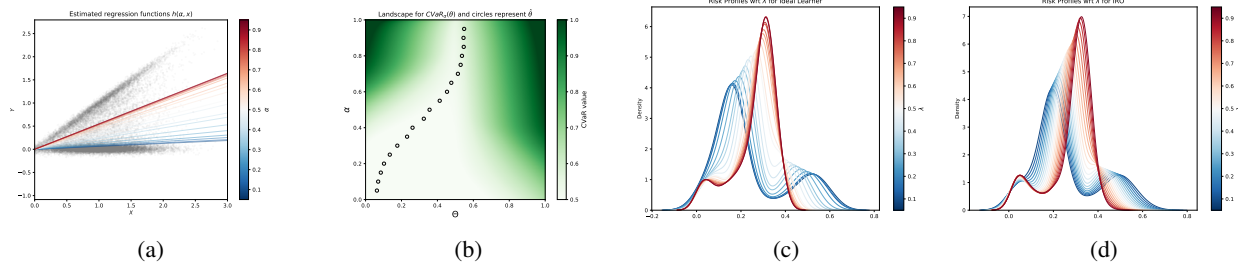
Figure 3: Figure 3a illustrated the data and the ideal learner f_\lambda(\hat{\theta}) \in \mathcal{H} for \lambda \in \{0.05, \dots, 0.95\} . Figure 3b describes the landscape of the objective function \rho (CVaR) for the ideal learner. We plot \hat{\theta} as circles. Figure 3c describes the Risk profile for \lambda \in \{0.05, \dots, 0.95\} for the ideal learner. Figure 3d describes the Risk profile for \lambda \in \{0.05, \dots, 0.95\} Imprecise Learner.
