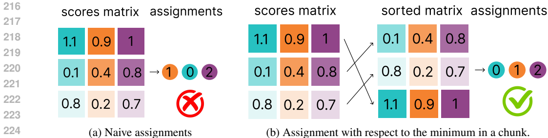
Figure 1: Balanced assignments. In this scenario we have 3 experts (columns with different colors) and 3 sequences to assign (rows) under the constraint that each expert should get 1 sequence. In (a) we assign sequentially each row, by negative log-likelihood, leading to sub-optimal assignment because the first expert is full when we try to assign the last row. On the other hand, in (b), we first sort wrt to the minimum log-likelihood which results in optimal assignments.
