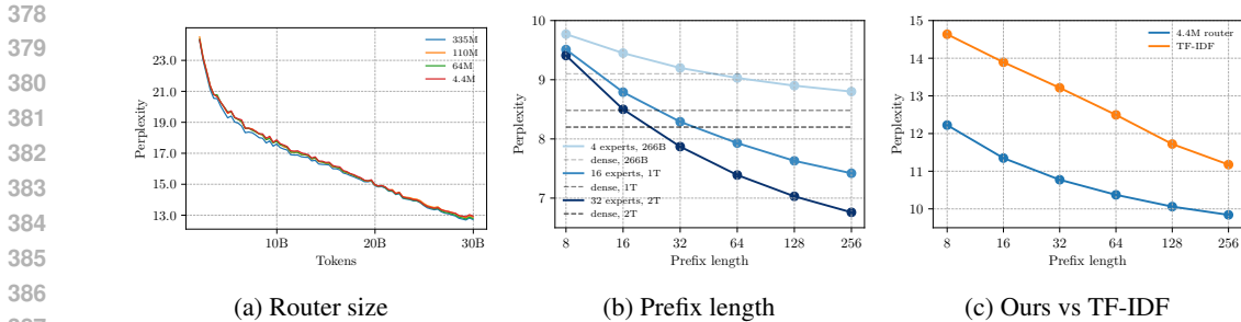
Figure 4: Routing analysis. (a) Test perplexity over training steps for different router sizes using a 335M parameter model with 4 experts. We compare routers of sizes 335M (where the model routes data for itself), 110M, 64M, and 4.4M parameters. (b) Test perplexity as a function of routing prefix length during inference for 1.3B parameter model with 4, 16 and 32 experts. We examine how reducing the prefix length \hat{M} used during inference affects performance when the data is partitioned during training using a prefix size M \geq \hat{M} . (c) Test perplexity over training steps for a 335M parameter model with 16 experts, comparing our proposed routing using TF-IDF document encoding followed by SVD projection and balanced K-Means clustering.
