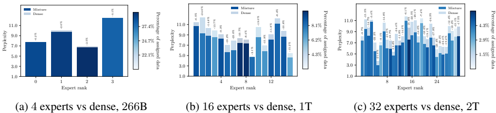
Figure 5: Experts Do specialize. Test perplexity comparison between our method and the dense baseline on the routed dataset segments for the 1.3B parameter model, using mixtures of 4 experts in (a) (trained on 266B tokens), 16 experts in (b) (1T tokens), and 32 experts in (c) (2T tokens). Each bar represents a dataset segment, with the color intensity indicating the percentage of data assigned to that expert – darker shades correspond to a higher proportion of data. Overlapping bars depict the perplexity achieved by the dense baseline (translucent) and our proposed mixture model (opaque). The results demonstrate that all experts specialize effectively on their assigned segments of the data distribution, leading to consistent improvements over the baseline. While the data distribution among experts is not perfectly even – with some experts receiving more data than others – all experts receive a substantial portion of the data. This shows that each expert contributes meaningfully to the overall performance gains.
