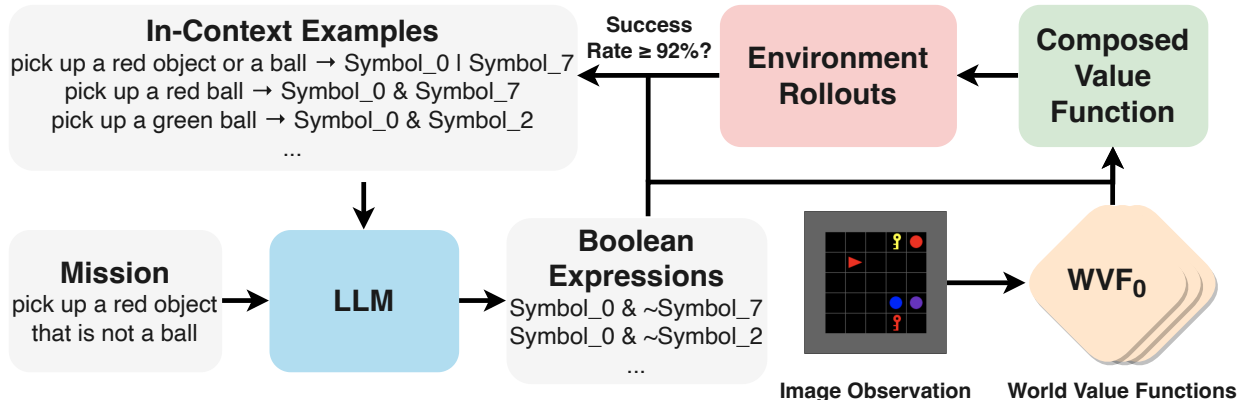
Figure 1: Pipeline diagram of the learning process for the CERLLA agent. The agent takes in a BabyAI language mission command and a set of 10 in-context examples are selected using the BM25 search retrieval algorithm (Robertson et al., 2009). The agent produces 10 candidate Boolean expressions. These expressions specify the composition of the base compositional value functions. Each compositional value function is instantiated in the environment and the policy it defines is evaluated over 100 rollouts. If the success rate in reaching the goal is greater than 92%, the expression is considered a valid parse of the language instruction and is added to the set of in-context examples.
