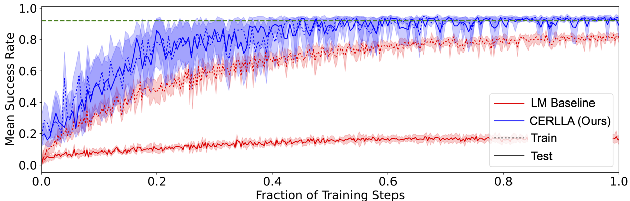
Figure 4: Results for learning on 81 randomly selected tasks and evaluating on the held-out 81 tasks. Learning curves are presented for our method and the baseline agents. The x -axis represents the fraction of the total training steps completed: 1 million for the CERLLA and 21 million for the LM Baseline agent. The dashed line denotes the success rate for considering the environment solved at 92%. Means and 95% confidence intervals are reported over 15 trials, 5 trials for the LM Baseline.
