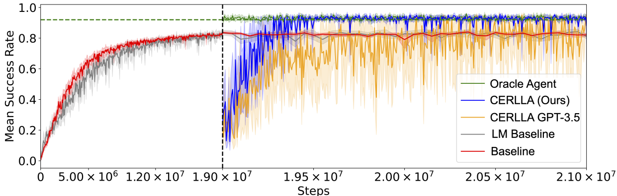
Figure 2: Results for learning all 162 tasks simultaneously. The mean episode success rate is plotted against the number of environment steps. Learning curves are presented for CERLLA and the non-compositional baseline agents. The Oracle agent is given the ground-truth Boolean expressions and upper bounds the attainable success rate in the environment, denoted by the dashed line at 92%. Our method is initialized at 19 million steps to reflect the number of training steps used in pretraining the compositional value functions. Note the change in steps scale at 19 million steps. Means and 95% confidence intervals are reported over 10 trials, 5 trials for the LM Baseline.
