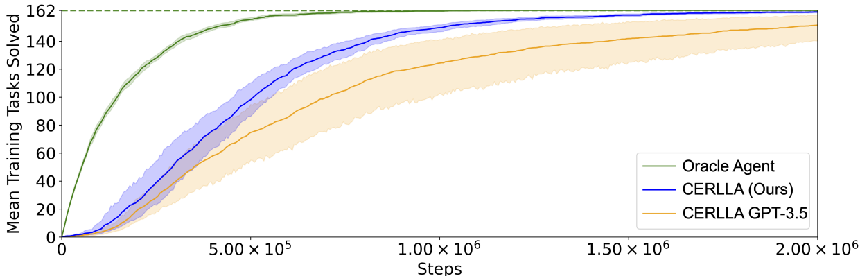
Figure 3: The mean number of tasks solved is plotted against the number of environment steps. This quantity is equal to the total number of in-context examples present in CERLLA’s in-context example set at that step. Because the Oracle Agent has access to the ground truth Boolean expressions for each task, it solves tasks immediately. The population of tasks remains constant, so the number of unsolved tasks decreases over time, leading to a logistic learning curve and an exponential decay in the rate at which new tasks are solved for the Oracle Agent. Means and 95% confidence intervals are reported over 10 trials.
