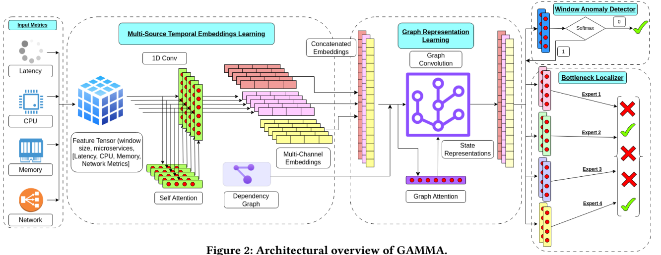
Figure 2: Architectural overview of GAMMA.
