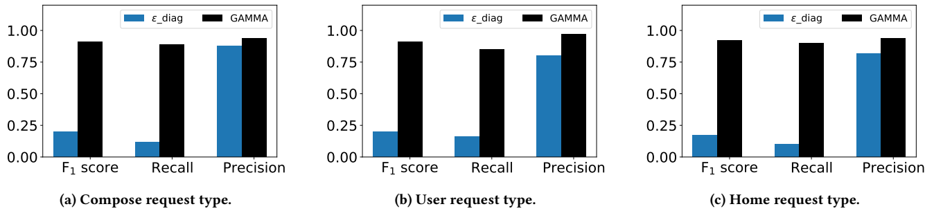
Figure 3: F1 score, Recall, and Precision for anomaly detection over the entire dataset.
