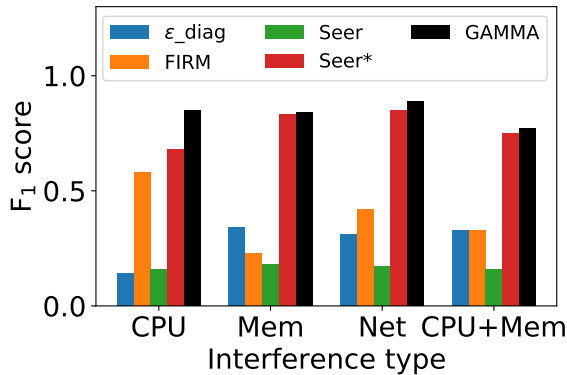
Figure 5: Bottleneck localization results by interference type.
