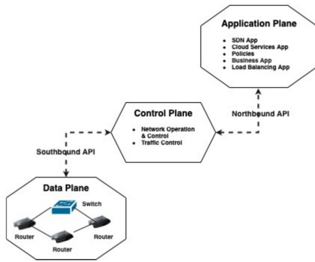
Figure 1: SDN Architecture
