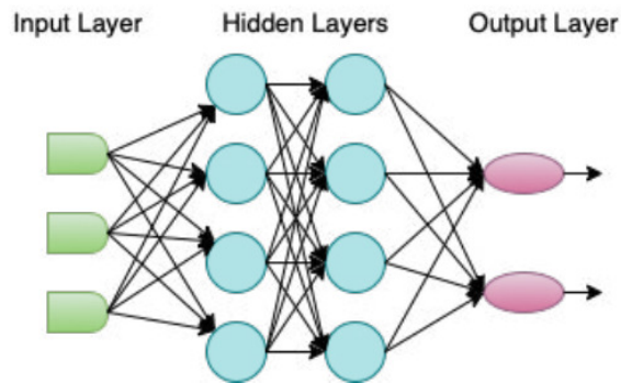
Figure 5: Multilayer perceptron
