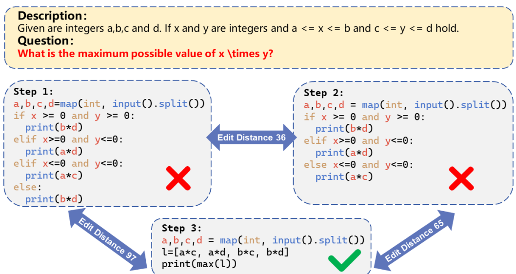
Figure 9: Case 2, an example of repair process for “Maximum possible value of x \times y ”.
