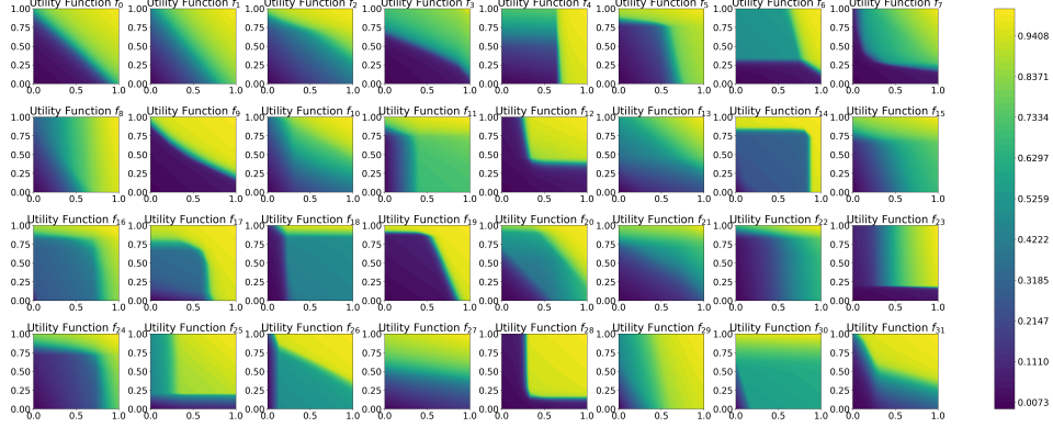
Figure 7: Illustration of 2D utility functions learned by our methods in Section 4.2.1.
