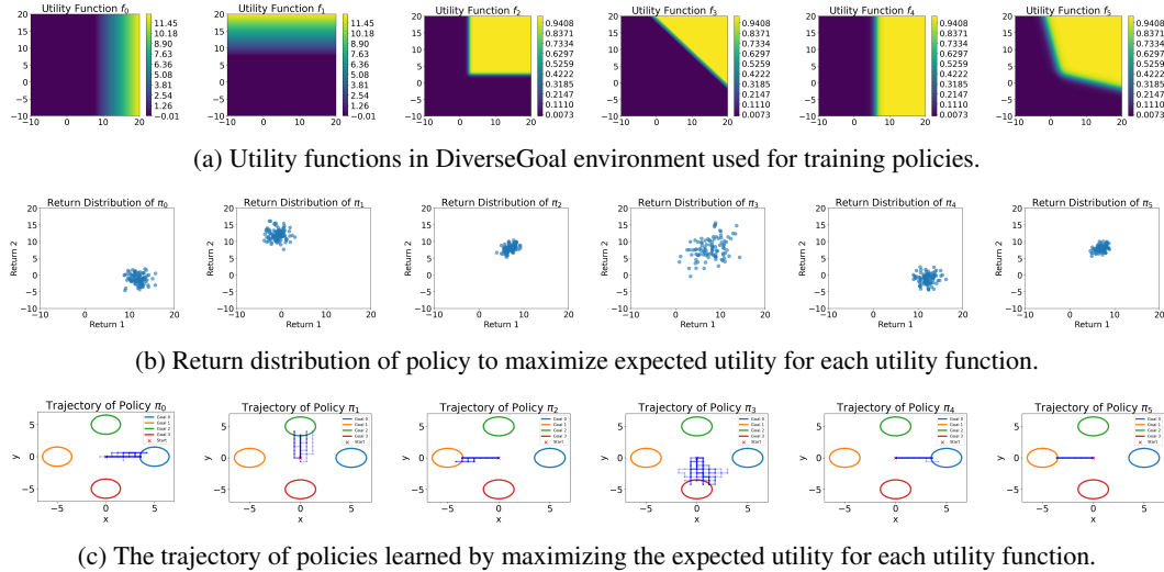
Figure 4: The case study results of DPMORL under DiverseGoal environment.
