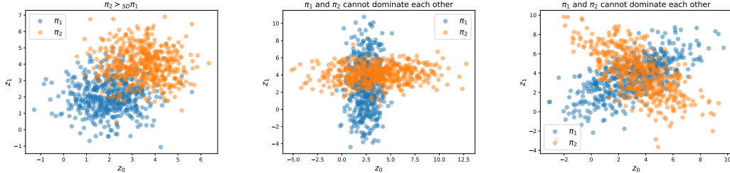
(a) Stochastic Dominance Example 1 (b) Stochastic Dominance Example 2 (c) Stochastic Dominance Example 3
