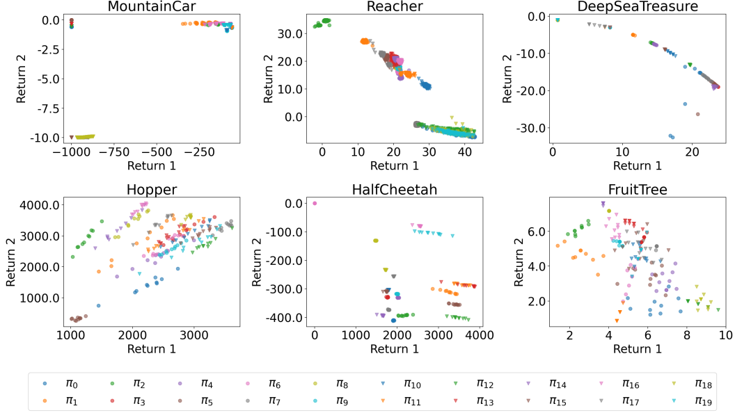
Figure 8: Return distribution of the set of policies learned by DPMORL on each environment.
