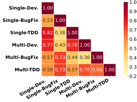
Figure 3: Pearson correlation matrix across six tasks.
