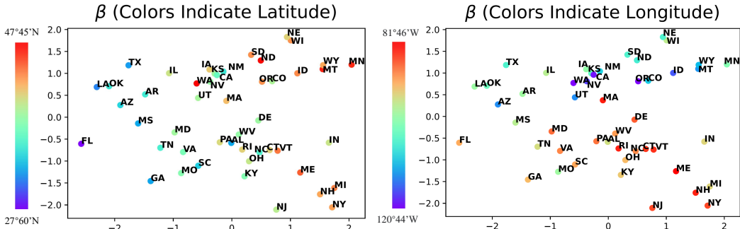
Figure 5: Inferred domain indices for 48 domains in TPT-48 . We color inferred domain indices according to ground-truth indices, latitude ( left ) and longitude ( right ). VDI 's inferred indices are correlated with true indices, even though VDI does not have access to true indices during training.
