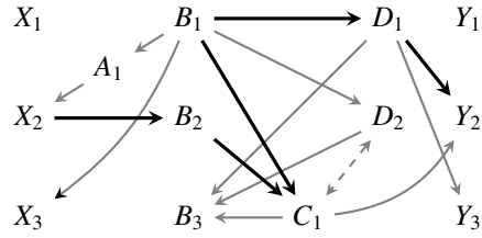
Figure 9: Figure 9a shows the graph \mathcal{G}^m containing the structure of interest \sigma^m (in bold black), which connects X^m and Y^m under C^m \cup A^m . Figures 9b, 9c and 9d illustrate the successive transformations of \mathcal{G}^m and \sigma^m (as carried out in the proof of Theorem 4) for the cluster B^C . Figure 9e shows the last step of the proof. Figure 9f shows how to transform the graph in Figure 9e to get the graph in Figure 3d.
