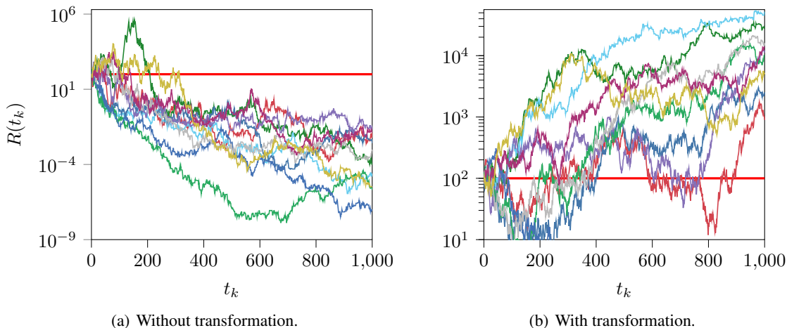
Figure 2. Learning bet strategies for the adapted coin toss game. Without transformation, most agents end up losing, while they end up winning with transformation.
