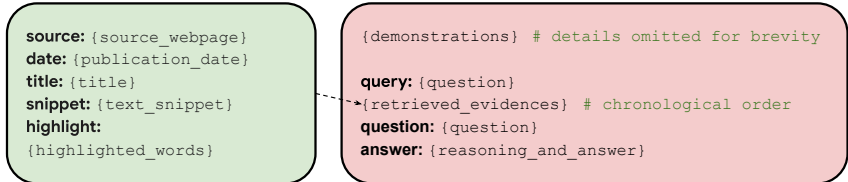
Figure 3: FRESHPROMPT’s format. We cast all retrieved evidences into a unified format with useful information, including source webpage, date, title, text snippet, and highlighted words (left). Few-shot demonstrations are provided at the beginning of the prompt. Each demonstration shows the model an example question and a list of retrieved evidences for the question, followed by some reasoning over the evidences to figure out the most relevant and up-to-date answer (right).
