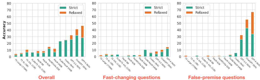
Figure 2: Accuracy of different LLMs on FRESHQA under RELAXED and STRICT (no hallucination) evaluations. Models benchmarked on the same date of April 26, 2023. All models (regardless of model size) struggle on questions that involve fast-changing knowledge and false premises .
