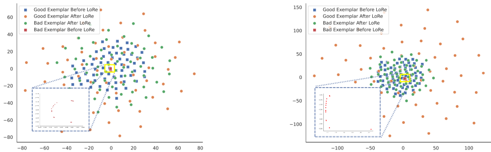
(a) The retriever is trained on the SVAMP dataset and tested on SVAMP, with results presented before and after LoRe.
