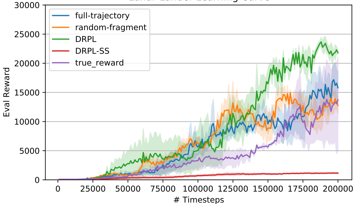
Lunar-Lander Learning Curve
