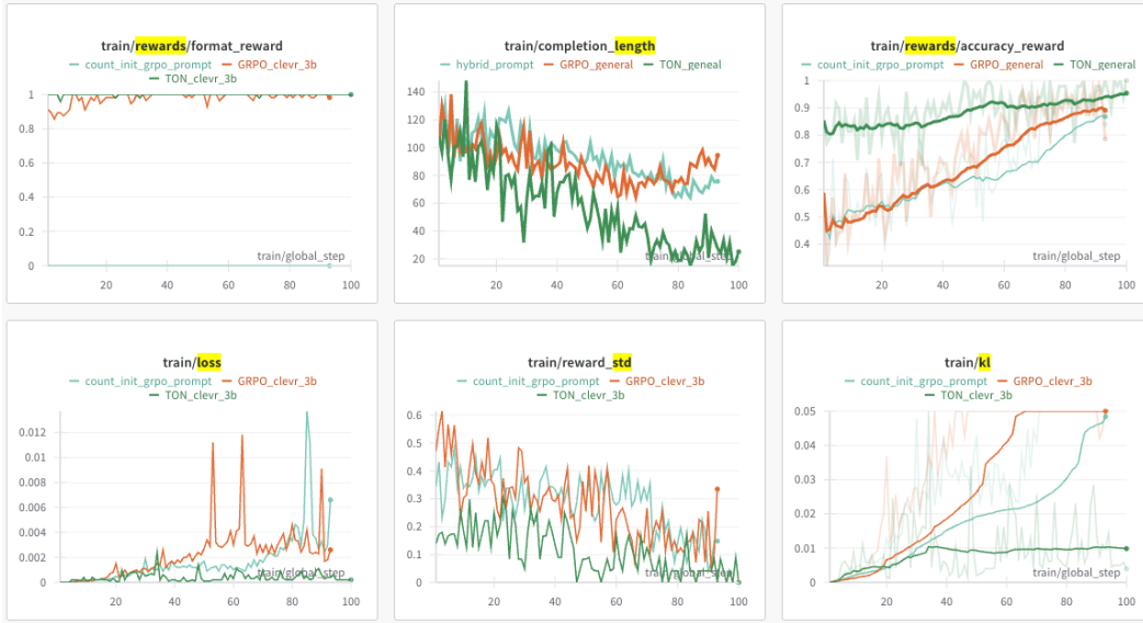
Figure 15: hybrid prompt v.s. SFT visualization during the training process on Qwen2.5-VL-3B on clevr.
