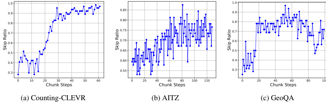
Figure 14: Skip Ratio of the output thinking during our TON training on three benchmarks.
