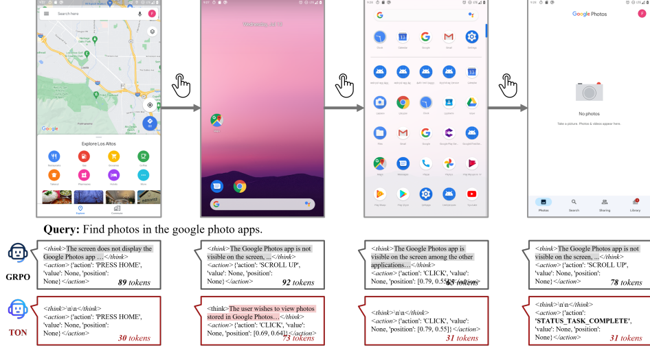
Figure 7: Comparison between GRPO and TON on Agent setting AITZ [13]. TON adaptively skips unnecessary think steps during multi-step mobile navigation, achieving greater decoding efficiency compared to GRPO while maintaining task accuracy (saving 60% tokens in this case).
