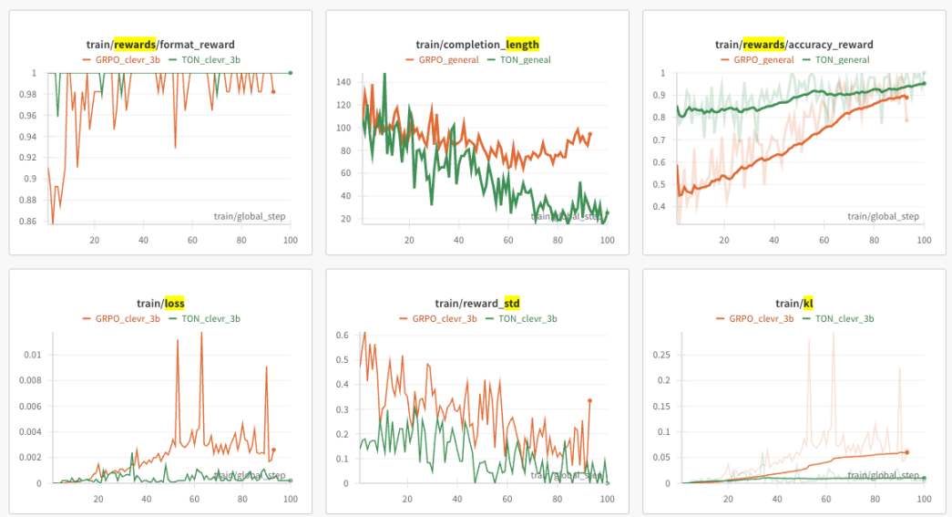
Figure 10: TON and GRPO visualization during the training process on Qwen2.5-VL-3B on CLEVR.
