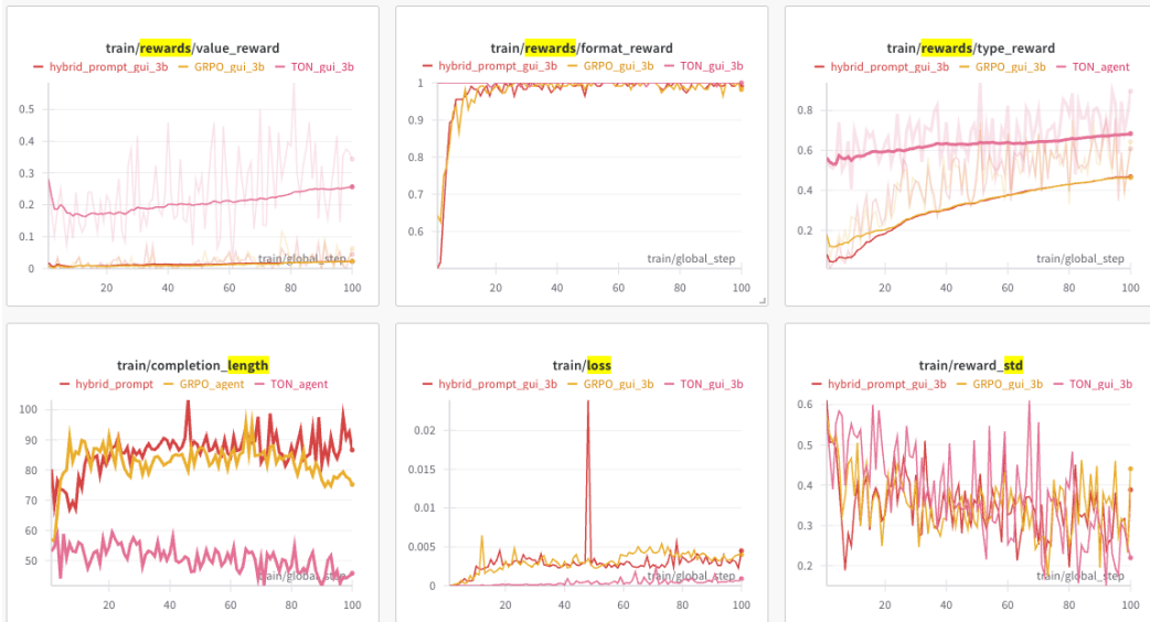
Figure 16: hybrid prompt v.s. SFT visualization during the training process on Qwen2.5-VL-3B on AITZ.
