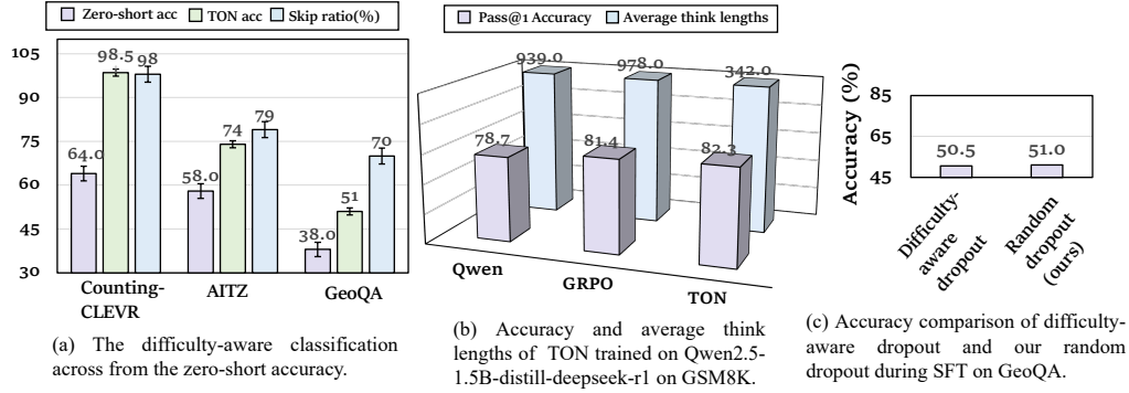
Figure 6: Further Analysis of TON. (a)(c) give the in-depth analysis of the effectiveness of our thought dropout and the generalization across the task difficulty. (b) shows the superiority of TON on the text-only domains.
