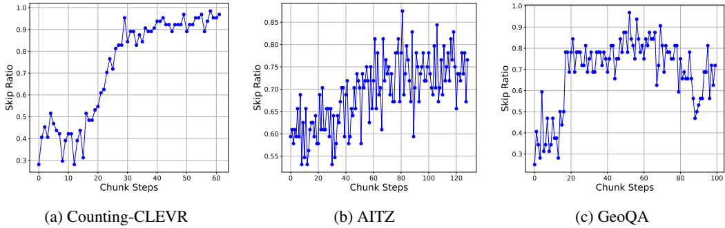
Figure 21: Skip ratio of the output thinking during our TON training on three benchmarks.
