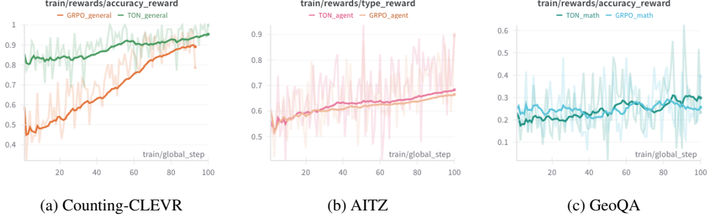
Figure 19: Rewards of the output during our TON training on three benchmarks.
