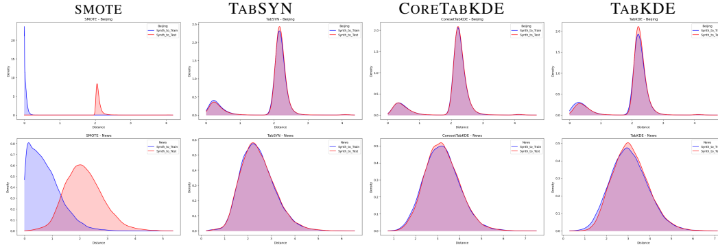
Figure 4: Privacy comparison based on DCR distributions for synthetic to training data (blue) and synthetic to held-out data (red). First row Beijing and second row News.
