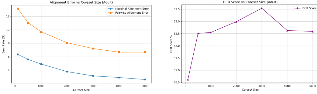
Figure 10: Left: Marginal distribution alignment error (%) and pairwise correlation alignment error (%) as coreset size increases. Right: DCR score as coreset size increases.
