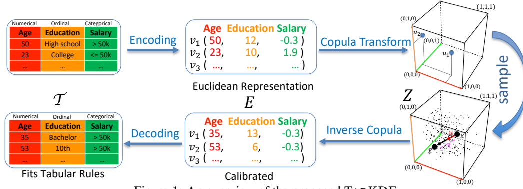
Figure 1: An overview of the proposed TABKDE.
