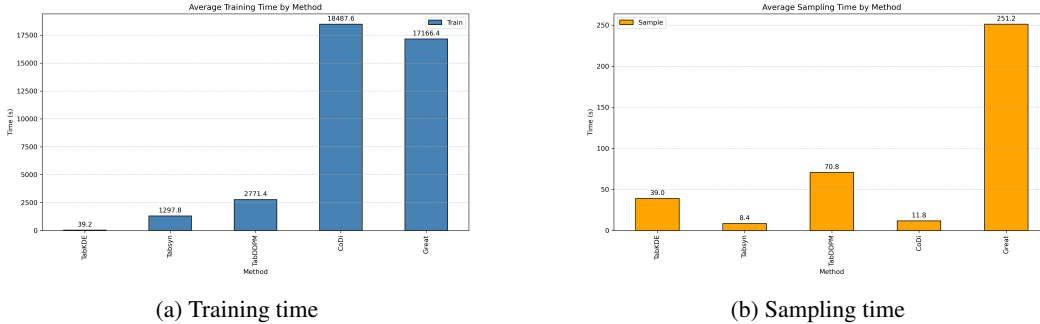
Figure 5: Average training and sampling time over Adult, Default, Shoppers, and Magic for different methods.
