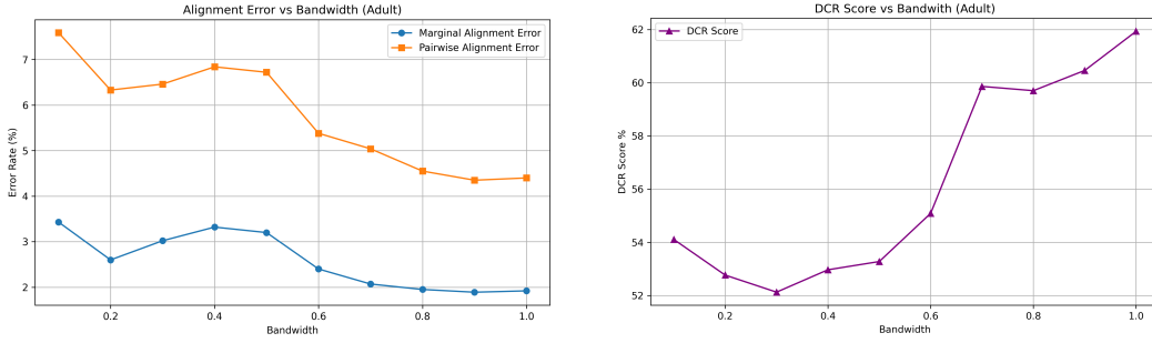
Figure 11: Left: Marginal distribution alignment error (%) and pairwise correlation alignment error (%) as bandwidth increases. Right: DCR score as bandwidth increases.
