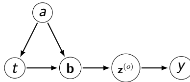
Figure 7. An SMCM signifying the importance of Assumption 2
