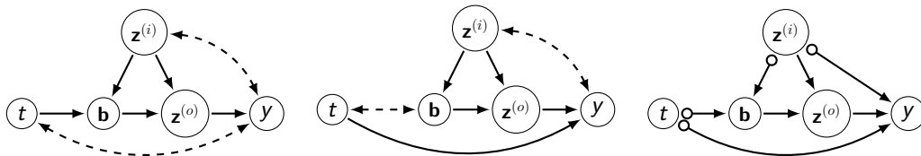
Figure 3. (a) An SMCM satisfying (5) and (6). (b) An SMCM obtained from (a) by modifying the edges between t and \mathbf{b} and between t and y . (c) The PAG corresponding to SMCM in (a) and (b).
