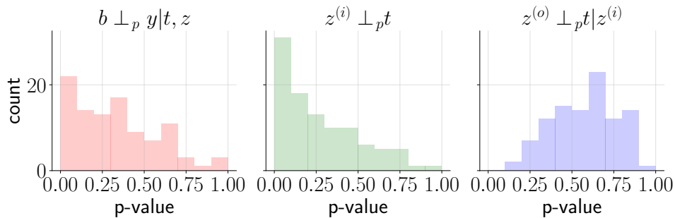
Figure 5. Histograms of p-values of the conditional independencies in (7) and (8) over 100 bootstrap runs for \mathbf{b} = \{\text{\# of people financially dependent on the applicant, applicant’s savings, applicant’s job}\} .
