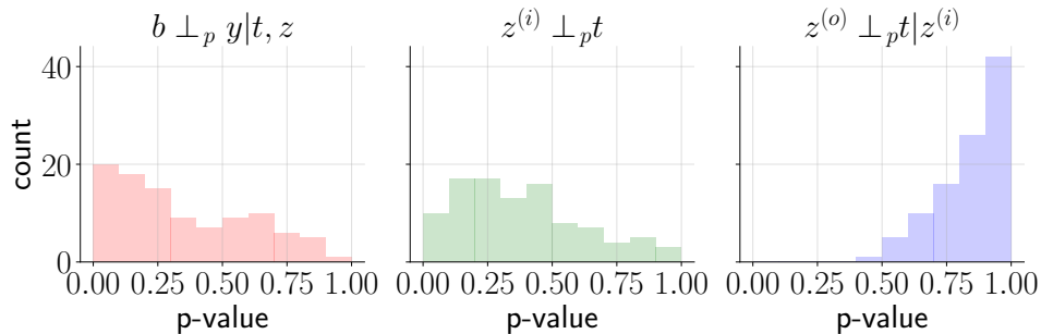
Figure 10. Histograms of p-values of the conditional independencies in (7) and (8) over 100 bootstrap runs for \mathbf{b} = \{\# \text{ of people financially dependent on the applicant, applicant's savings}\} , Algorithm 1 results in \mathbf{z}^{(i)} = \{\text{purpose for which the credit was needed, applicant's checking account status with the bank}\} .
