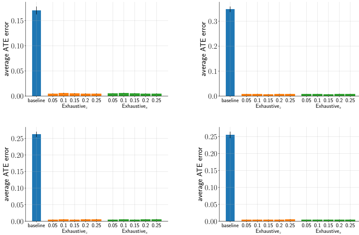
Figure 9. Performance of Algorithm 1 for different p-value thresholds p_v on \mathcal{G}^{toy} in Figure 2 on top left, on \mathcal{G}_1^{toy} from Figure 8 on top right, on \mathcal{G}_2^{toy} in Figure 8 on bottom left, and on \mathcal{G}_3^{toy} from Figure 8 on bottom right
