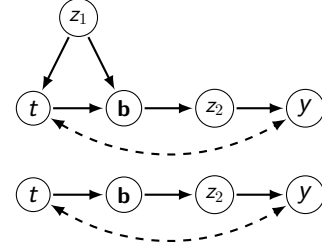
Figure 6. SMCMs on (top) & (bottom) satisfy \mathbf{b} \perp\!\!\!\perp_d y|t, \mathbf{z} but have different causal effect estimation formulae.
