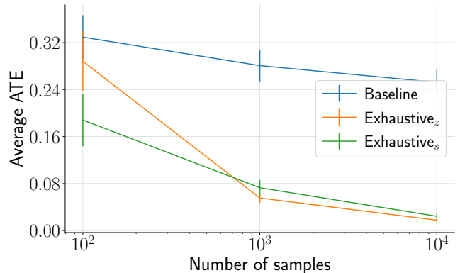
Figure 4. Average ATE for Algorithm 1 and Baseline vs. number of samples.
