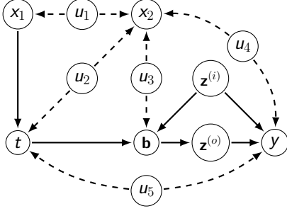
Figure 2. The graph \mathcal{G}^{toy} satisfying Assumptions 1 to 3 where u_i are unobserved.
