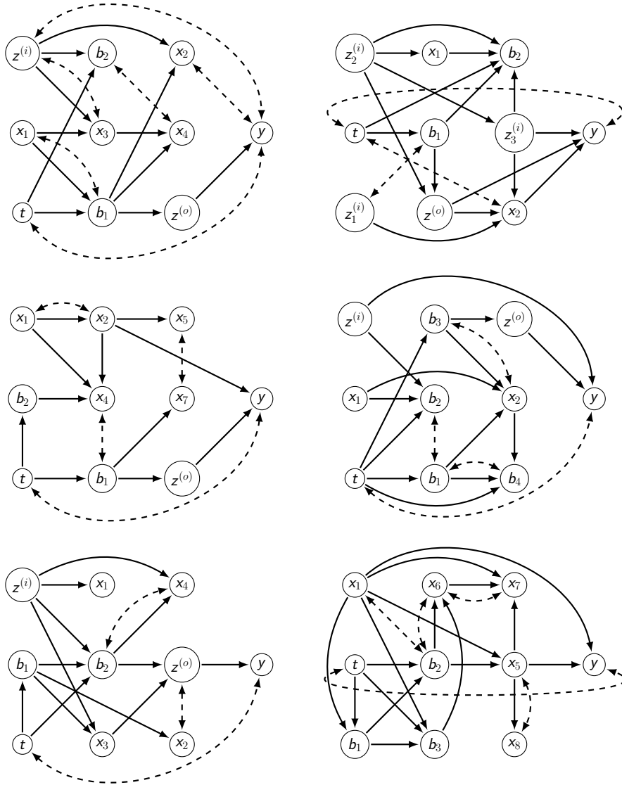
Figure 11. The SCMs used in Appendix D.2 to compare Algorithm 1 with the Baseline that uses \mathbf{b} for front-door adjustment. These are the 6 out of the 100 random graphs in Appendix D.1 for p = 10 , d = 2 , and q = 1.0 where our approach was successful indicating existence of \mathbf{z} = (z^{(i)}, z^{(o)}) such that the conditional independence statements in Theorem 3.2 hold.
