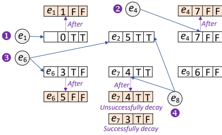
Figure 2: Running examples of Pontus's update process.
