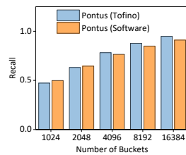
Figure 5: Recall rate on hardware and software platforms.
