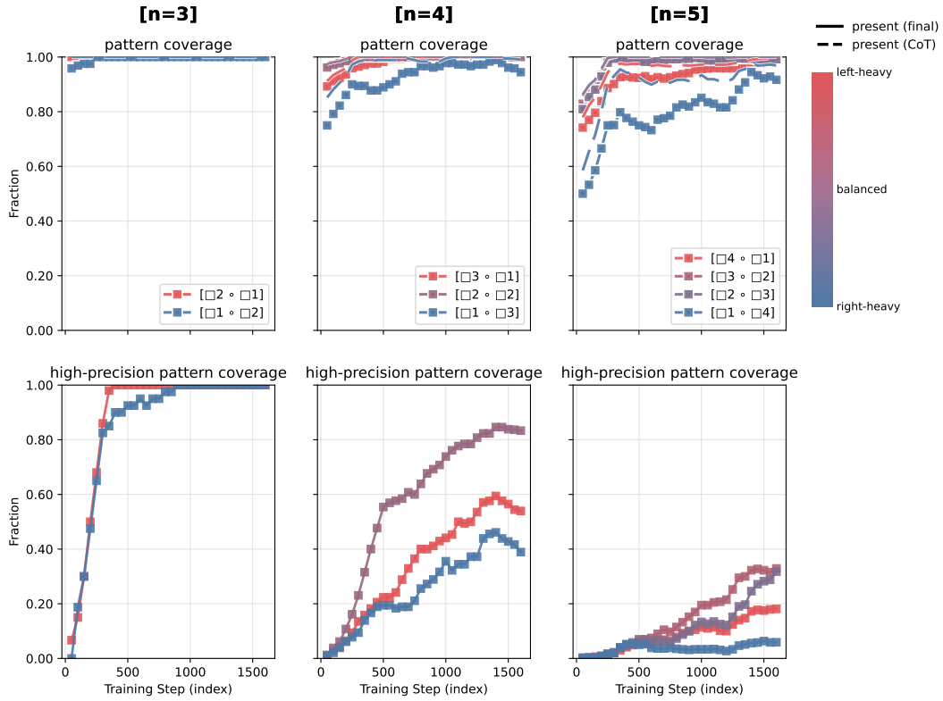
Figure 15: Learning dynamics at a glance (Qwen2.5-1.5B) with reversed canonicalization. The same conclusion from Figure 3 holds about the hierarchy of difficulty by subtree structure: balanced < left-heavy < right-heavy.
