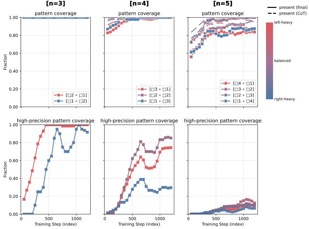
Figure 14: Learning dynamics at a glance (Llama-3.2-3B after lightweight SFT) . The same conclusion from Figure 3 holds about the hierarchy of difficulty by subtree structure: balanced < left-heavy < right-heavy.
