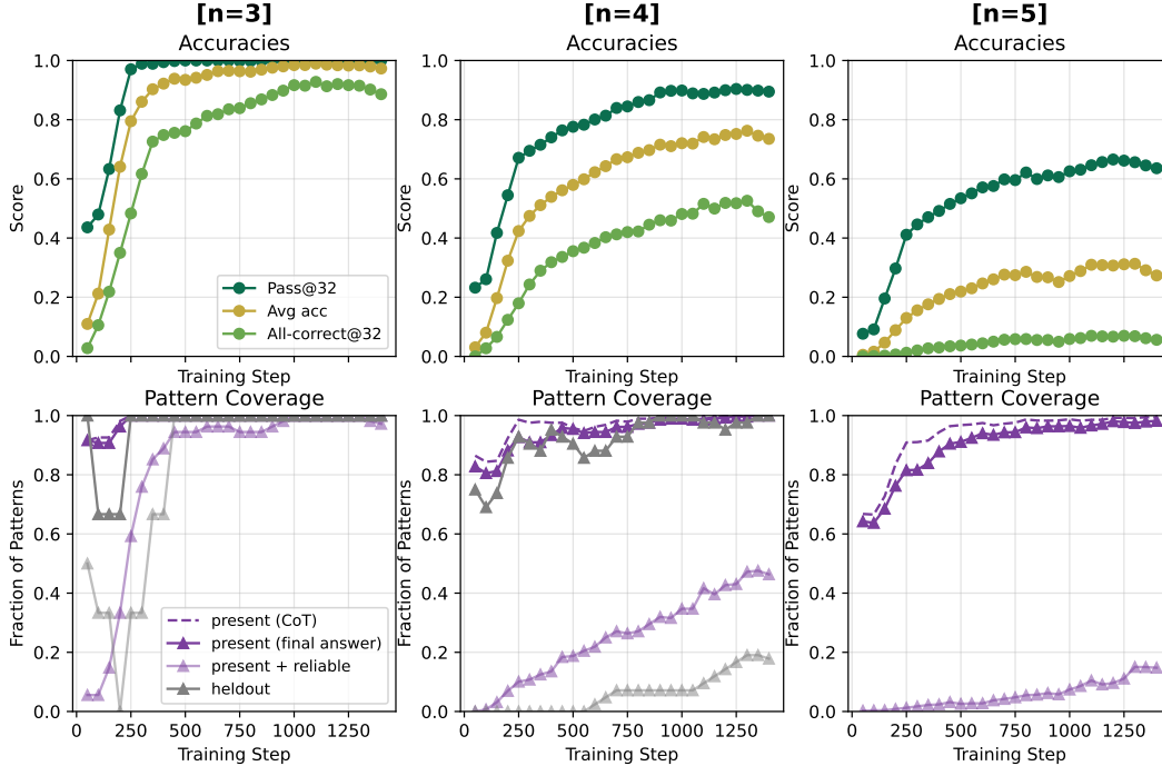
Figure 4: Generalizes to entire families of held-out compositional patterns. To evaluate compositional generalization, we removed an entire family of related patterns from the training set: the base n = 3 structure A/B + C and all of its n = 4 extensions (e.g., A/B + C + D , A/(B + C) + D ). The model successfully recovers these unseen patterns. Coverage first emerges on the held-out n = 3 subpattern before generalizing to its more complex n = 4 dependents, matching the typical learning hierarchy where presence precedes precision. This result demonstrates that the model can reuse learned substructures to assemble novel operator-tree shapes it has never been explicitly trained on.
