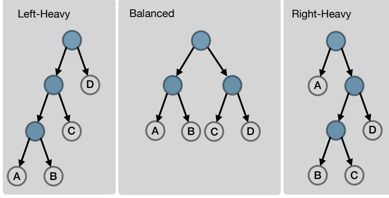
Figure 5: Grouping canonical patterns by tree structure ( n = 4 ). Internal (blue) nodes are operators and leaves ( A, B, C, D ) are operands. We categorize patterns by the relative size of the root's subtrees: left-heavy, balanced, or right-heavy.
