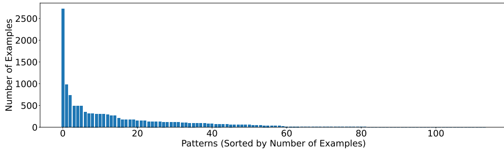
Figure 6: Number of examples per pattern in Pan et al. [2025b]. 18 out of 114 patterns do not appear in a randomly selected 10000 examples from the dataset. Few patterns (mostly from n = 3 ) appear disproportionately frequently.
