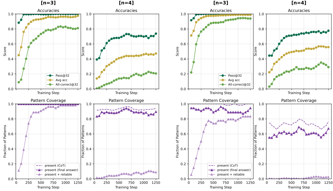
Figure 7: Learning dynamics at a glance (Qwen2.5-3B) trained on dataset from Pan et al. [2025a]. (Left) evaluated on our dataset; (Right) evaluated on the held-out data from Pan et al. [2025a]. Even though model accuracy smoothly increases (top), models do not reliably learn most n = 4 patterns and fails to generate at least 10% of n = 4 patterns (bottom). The held-out data from Pan et al. [2025a] do not include 36 possible patterns and fail to test the models on the corresponding skills.
