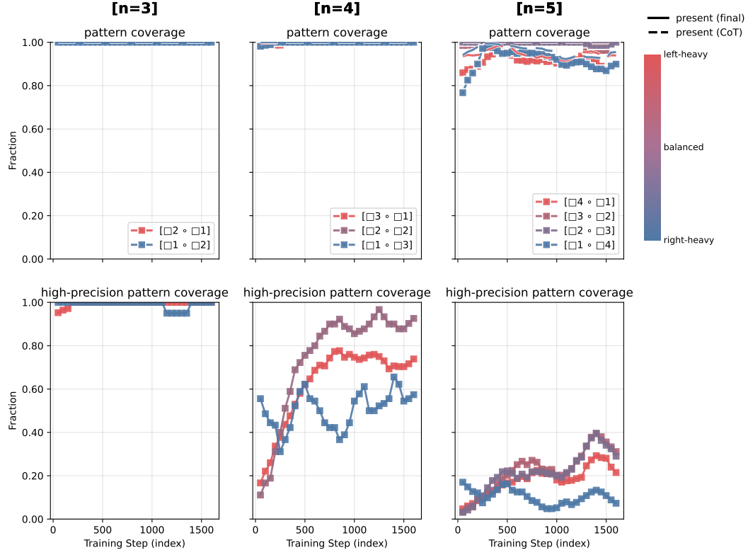
Figure 18: Learning dynamics at a glance (Qwen2.5-7B) . The same conclusion from Figure 3 holds about the hierarchy of difficulty by subtree structure: balanced < left-heavy < right-heavy.
