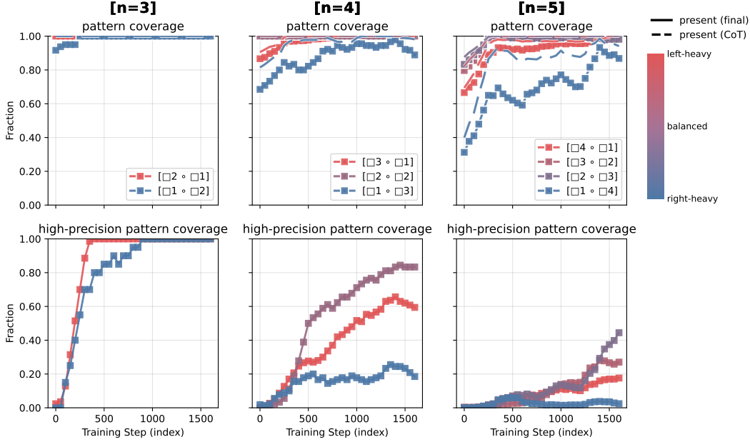
Figure 3: Compositional structure (not input length) determines difficulty. Within n = 4 , balanced patterns ( [2] \circ [2] ; purple) are discovered (top row) and mastered far more reliably (bottom row) than the unbalanced ones (red/blue). Balanced patterns have shallow trees, with solution depth of 2 equal to that of n = 3 puzzles. Even when controlling for depth, right-heavy patterns ( [1] \circ [3] ; blue) are substantially harder than left-heavy patterns ( [3] \circ [1] ; red). This evidence points to a “lookahead bottleneck” suggesting that a primary failure mechanism is the challenge of committing to a solution ahead of a complex subroutine. The entire structural hierarchy persists for n = 5 .
