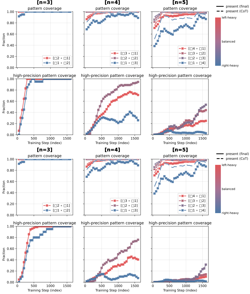
Figure 20: Learning dynamics at a glance (Qwen2.5-1.5B) but high-precision defined as precision \geq 70\% (top); \geq 90\% (bottom). The same conclusion from Figure 3 holds about the hierarchy of difficulty by subtree structure: balanced < left-heavy < right-heavy.
