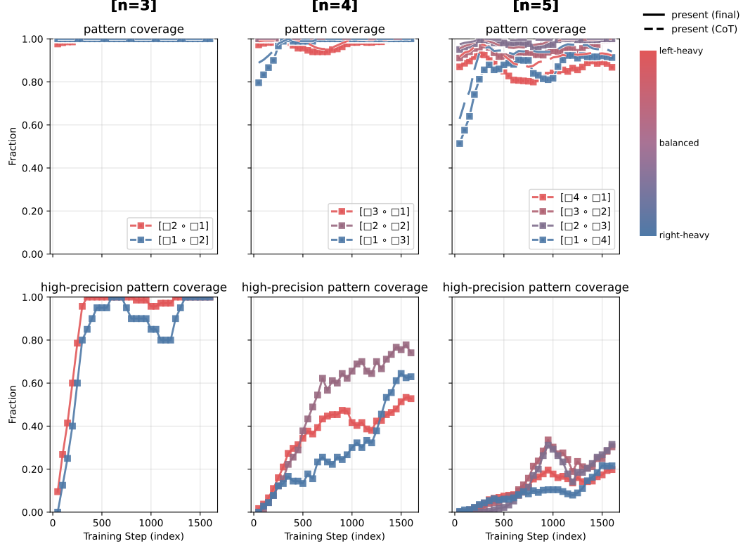
Figure 17: Learning dynamics at a glance (Qwen2.5-3B) . The same conclusion from Figure 3 holds about the hierarchy of difficulty by subtree structure: balanced < left-heavy < right-heavy.
