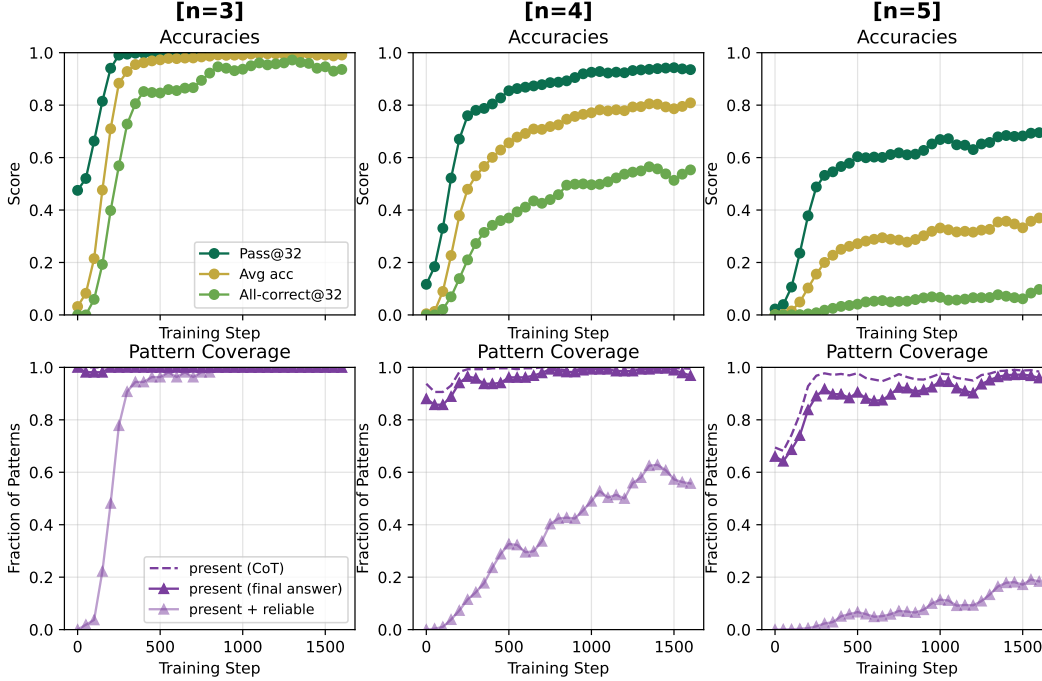
Figure 2: Successful length generalization, but a gap between pattern discovery and reliable execution. We train Qwen2.5-1.5B on problem sizes n \in \{3, 4\} and evaluate on held-out data for n \in \{3, 4, 5\} . (Top) The model demonstrates strong length generalization : accuracy on the held-out n = 5 problems improves substantially with training. (Bottom) The model also identifies almost all compositional patterns for n = 5 , but the ability to reliably execute the correct pattern lags significantly behind its discovery. This indicates that the primary challenge for generalization is procedural reliability, not abstract pattern identification.
