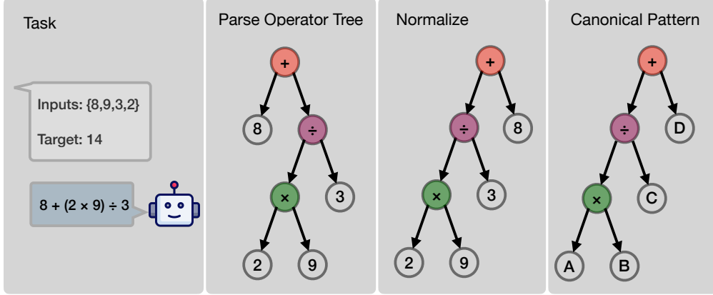
Figure 1: From generated expression to canonical pattern. The model-generated expression 8 + (2 \times 9) \div 3 is parsed into an expression tree, normalized with respect to algebraic identities, and mapped to the unique canonical pattern A \times B \div C + D . Patterns are then grouped by their computational shape. Here, the root operator is “+”, with a left sub-expression over three leaves ( A, B, C ) and a right sub-expression over one leaf ( D ). The signature [3] + [1] serves as a compact representation of the pattern’s structure at the root-level.
