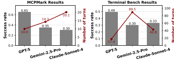
Figure 8: Benchmark results on MCPMark (Postgres subset) and Terminal-Bench (subset) using GEM as a unified evaluation toolkit.
