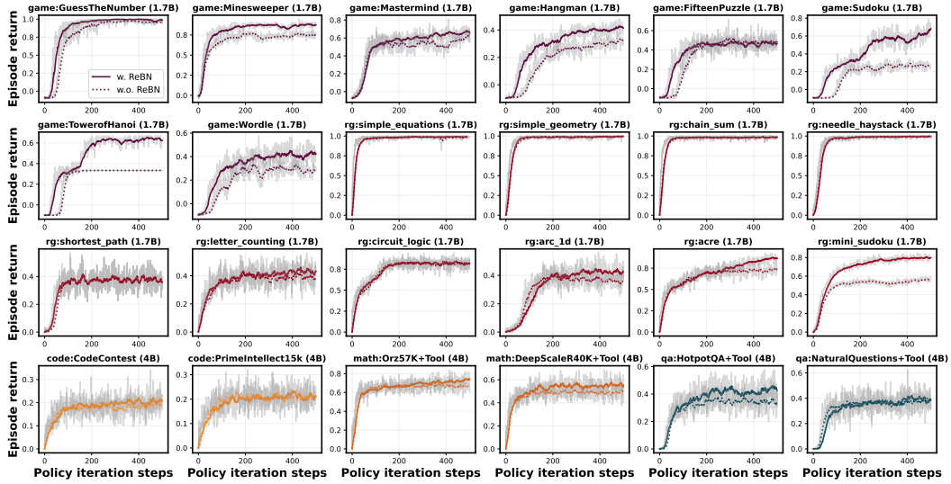
Figure 1: Learning curves of Qwen3-based agents across diverse environments of 5 categories: game (language games); rg (ReasoningGym); code (coding tasks); math (python-integrated math questions); qa (search-integrated general questions). All agents are learned via a simple yet general multi-turn algorithm based on REINFORCE (Algorithm 1). The comparison between two curves in each subplot illustrate the effectiveness of Return Batch Normalization (ReBN).
