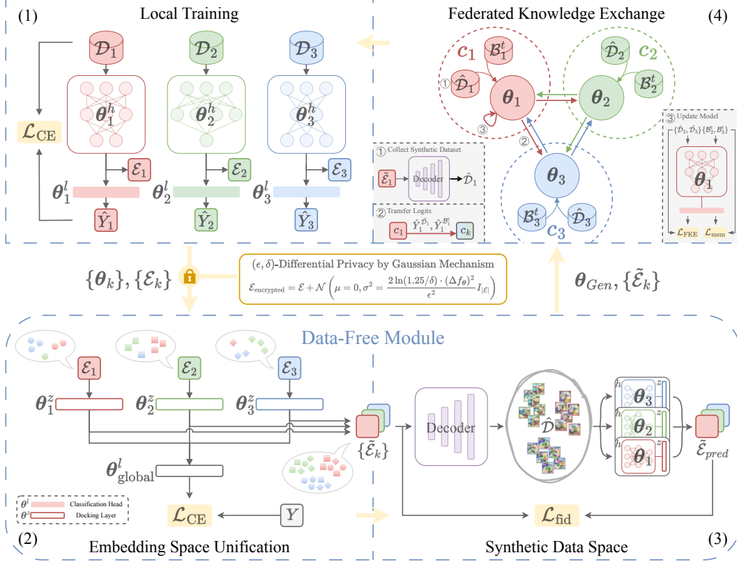
Figure 2: DFFKE comprises four procedures per communication round: (1) Training on each client’s private dataset to prepare for knowledge sharing, (2) Translating each client’s embeddings distribution into a unified embedding space, (3) Training an emb-decoder to map the unified embedding space to the data space, and (4) Conducting FKE using synthetic transfer data and a memory buffer.
