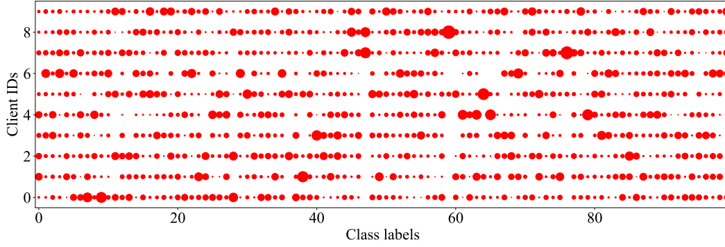
Figure 6: 10 Clients, CIFAR100, Low Data-Hetero ( \alpha = 1.0 )
