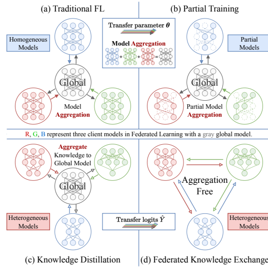
Figure 1: Comparison of three general approaches in Federated Learning with FKE.
