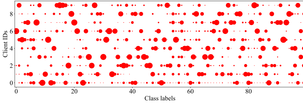
Figure 7: 10 Clients, CIFAR100, High Data-Hetero ( \alpha = 0.1 )
