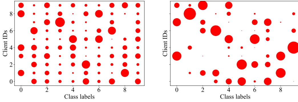
Figure 5: Left: 10 Clients, CIFAR10, Low Data-Hetero ( \alpha = 1.0 ). Right: 10 Clients, CIFAR10, High Data-Hetero ( \alpha = 0.1 ).
