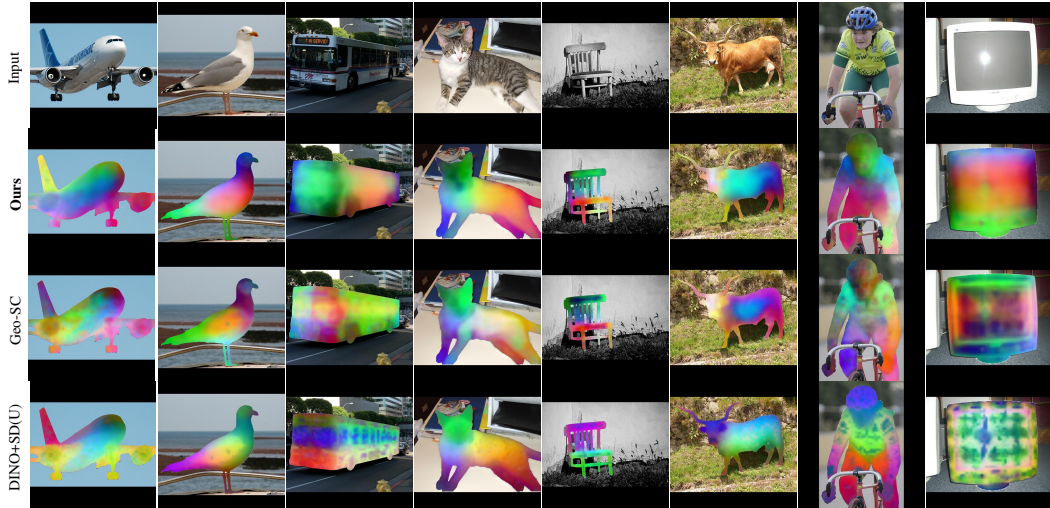
Figure 4: PCA visualization of the feature maps from different models. Note that PCA is computed on object features only. The inclusion of geometric constraints during training results in fewer high frequency artifacts in the predicted feature maps for our approach.
