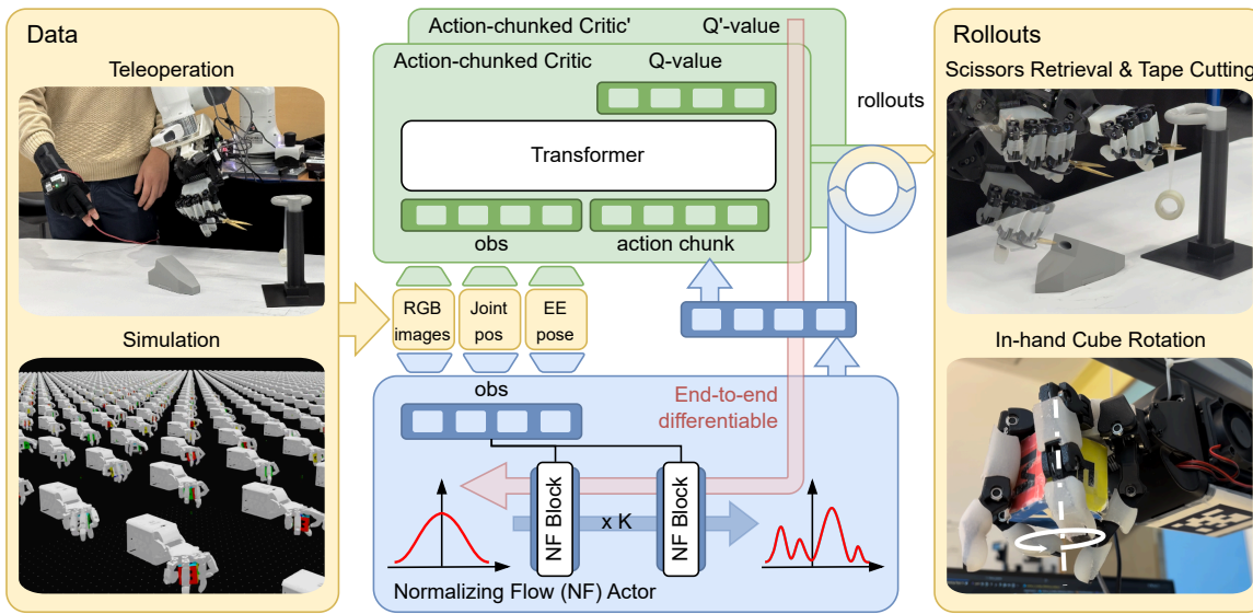
Fig. 1. Overview of SERNF (Sample-Efficient Reinforcement Learning with Normalizing Flows). SERNF models action chunks using a conditional normalizing flow policy, enabling expressive multimodal action distributions with exact likelihoods and therefore allowing direct, conservative off-policy fine-tuning. An action-chunked critic evaluates entire action sequences, aligning value estimation with chunked execution and improving long-horizon credit assignment. Initialized from real-world teleoperation data or policies trained in simulation, SERNF achieves high real-world performance under a limited interaction budget, demonstrating stable and sample-efficient adaptation on challenging dexterous manipulation tasks.
