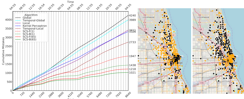
Figure 1: Left: Mean cumulative mistakes over 25 iterations for all algorithms and benchmarks over 48 hours (8640 trials) on a 404-vertex graph. A comparison of the mean performance of SCS with bases \mathcal{F}_n and \mathcal{B}_n (SCS-F and SCS-B respectively) using an ensemble of size 1 and 65 is shown. Right: An example of two binary labelings taken from the morning and evening of the first 24 hours of data. An ‘orange’ label implies that station is < 50\% full and a ‘black’ label implies that station is \geq 50\% full.
