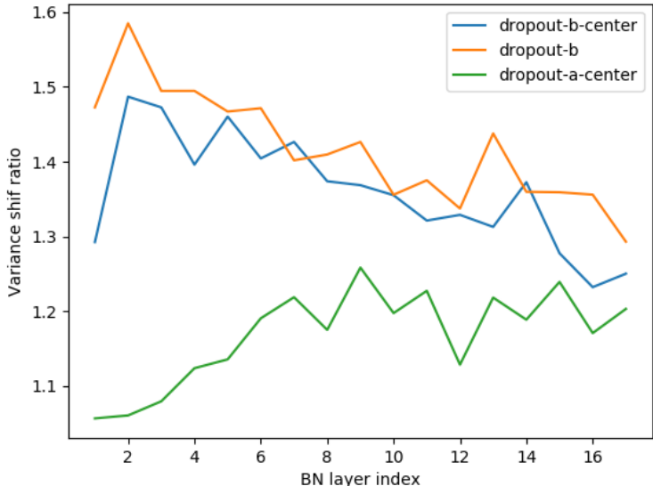
Figure 2: The variance shift ratio for differet dropout variants in the 18 residual blocks from ResNet110, the third residual stage. Lower values are better.
