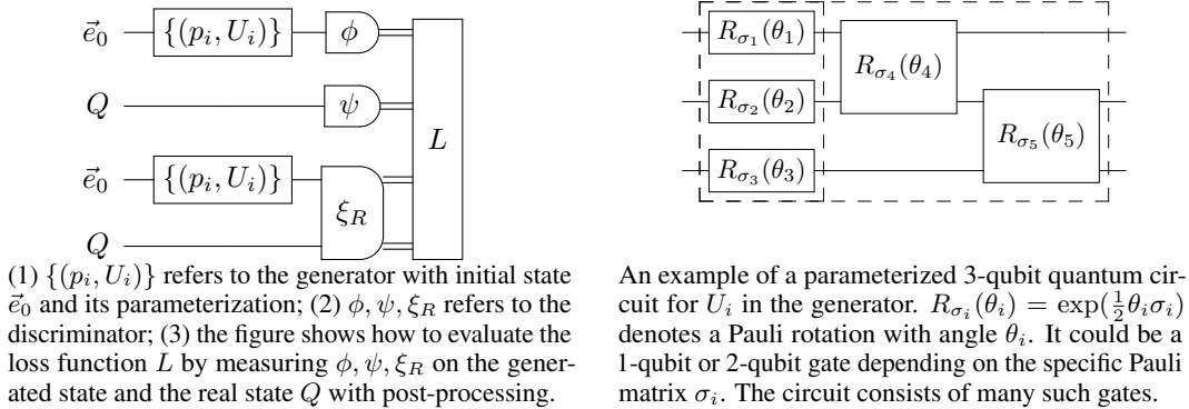
Figure 1: The Architecture of Quantum Wasserstein GAN.
