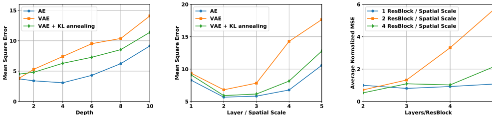
Figure 1: Reconstruction errors for various encoder/decoder models of varying complexity. Left : Fully connected networks with different depths trained on Fashion-MNIST. Middle : Convolution networks with increasing depth/# of spatial scales trained on Cifar100. Right : Averaged AE results from residual networks with varying number of residual blocks and block depth trained on SVHN, Cifar10, Cifar100 and CelebA. In all plots, once the encoder/decoder complexity is sufficiently high, the reconstruction errors begin to increase.
