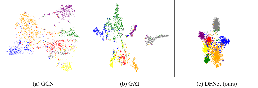
Figure 5: The t-SNE visualization of the 2-D node embedding space for the Cora dataset.
