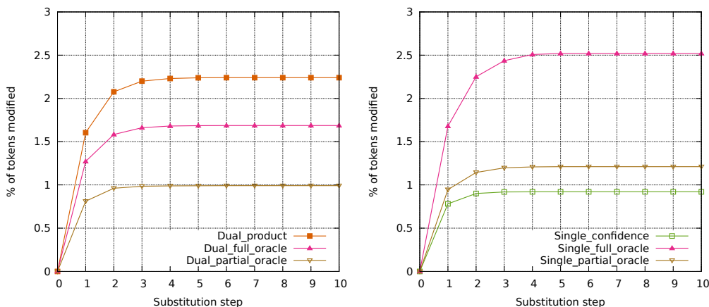
Figure 3: Percentage of modified tokens as a function of total number of substitutions allowed per sentence for the dual attention model (left) and the single attention model (right) compared to the full and partial oracles (cf. Figure 2).
