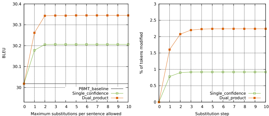
Figure 1: Left : BLEU as a function of the total number of substitutions allowed per sentence. Values are reported on a small 3K validation set for the single and dual attention models using the best scoring heuristic s and threshold t . Right : Percentage of modified tokens on the validation set as a function of the total number of substitutions allowed per sentence. All models modify fewer than 2.5% of tokens.
