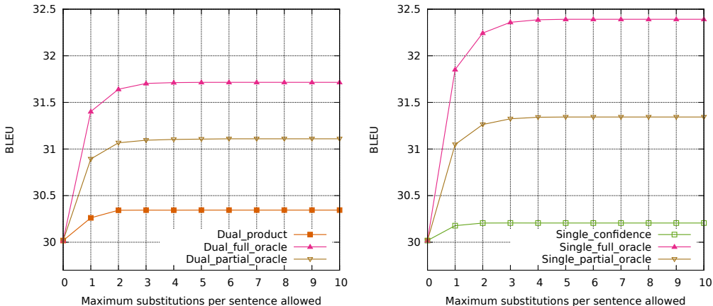
Figure 2: BLEU as a function of the total number of substitutions allowed per sentence. Left : best dual-attention refinement strategy (Dual_product) versus two oracles. The full oracle (Dual_full_oracle) accepts as input y_{pred} and selects a single i to substitute y_g^i := y_{pred}^i . The partial oracle (Dual_partial_oracle) lets the model choose position as well ( i := \arg \max_{1 \leq j \leq |y_g|} s(y_g, y_{pred}^j) ) but has the ability to prevent substitution y_g^i := y_{pred}^i if it does not improve BLEU. Right : same for the best single attention setup.
