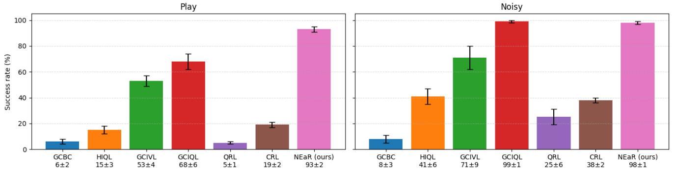
Fig. 2. Success rates on cube-single under play and noisy datasets. Comparison of NEaR with imitation-based (GCBC) and representative goal-conditioned value-based baselines. On play , NEaR achieves 93\% \pm 2 , substantially outperforming behavioral cloning and exceeding value-based methods. On noisy , NEaR reaches 98\% \pm 1 , closely matching GCIQL ( 99\% \pm 1 ). Results are averaged over evaluation seeds; error bars denote standard deviation.
