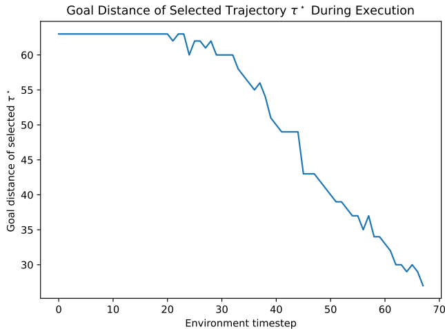
Fig. 5. At each environment timestep, NEaR selects the candidate trajectory \tau^* = \arg \min_\tau E_\theta(\tau) . The plot shows the distance between the goal token index t_g of trajectory \tau^* as execution proceeds. Goal distance decreases almost monotonically, demonstrating that energy-guided refinement produces progressively more goal-aligned plans. Example empirical rollout.
