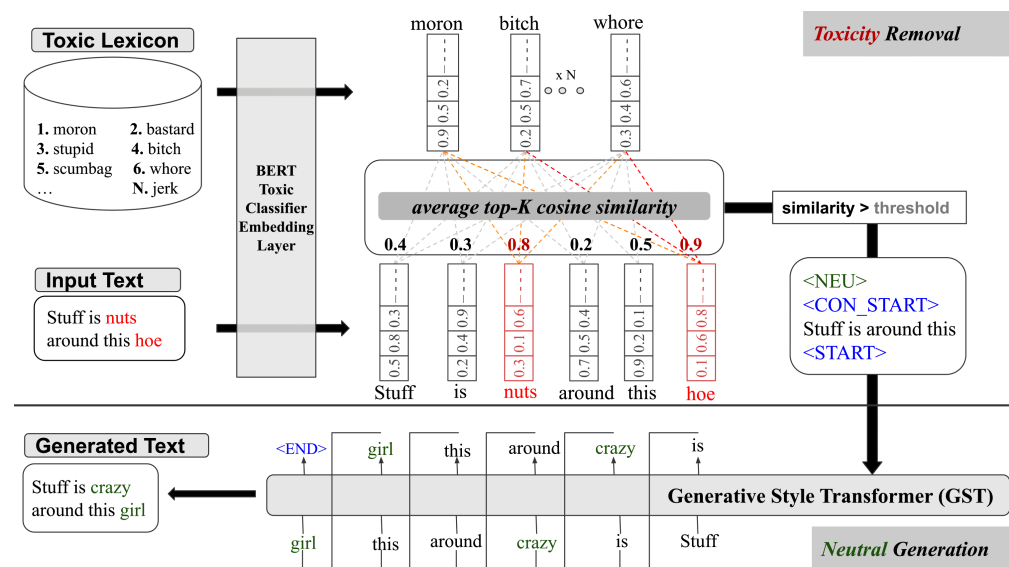
Figure 1. LexiconGST architecture.
