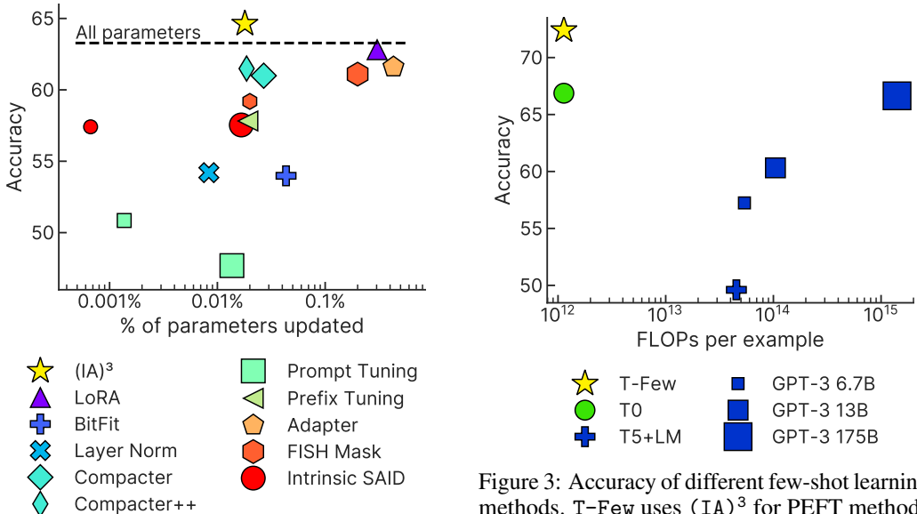
Figure 2: Accuracy of PEFT methods with L_{UL} and L_{LN} when applied to T0-3B. Methods that with variable parameter budgets are represented with larger and smaller markers for more or less parameters.
