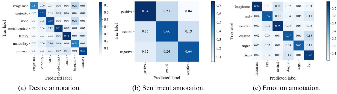
Figure 3: The confusion matrices show the annotations difference between different labels for three tasks.
