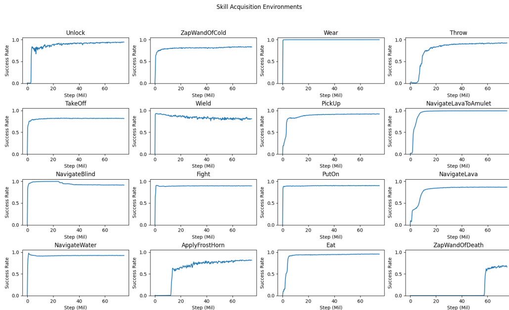
Figure 10: Success rate for training skill experts on the 16 skill acquisition environments
