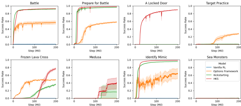
Figure 4: Success rate for all methods on the 8 SkillHack tasks, averaged over the repeats of each experiment. The shaded area denotes 1 standard error.
