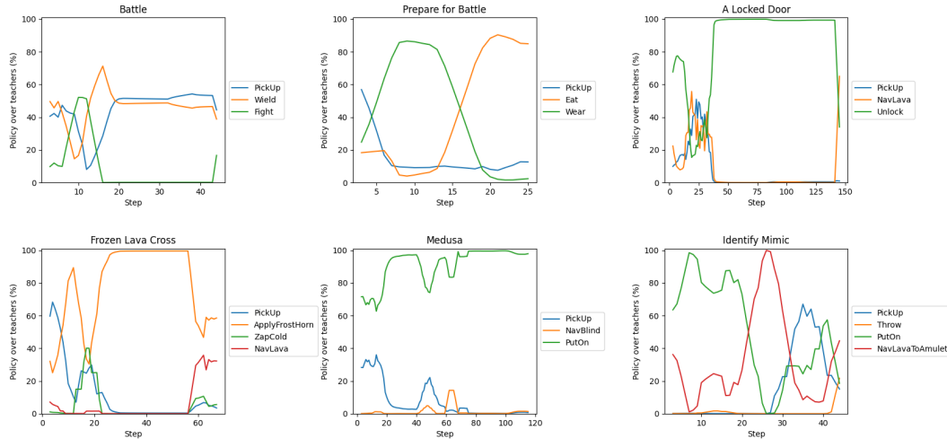
Figure 5: Distribution of policy-over-teachers for converged HKS policies over the span of a single episode. Results are each taken from a single successful run, smoothed with a rolling average of 6 timesteps. Note that the sampled FROZEN LAVA CROSS had a Frost Horn spawn. Only the 6 environments in which HKS converged on are shown.
