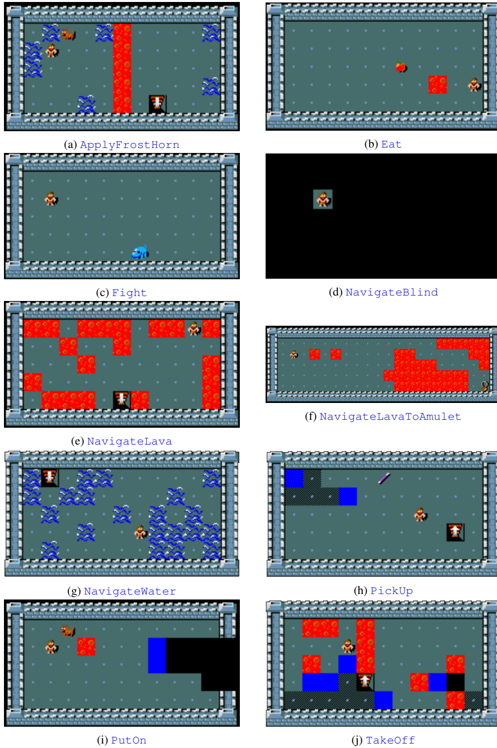
Figure 6: Skill environments.
