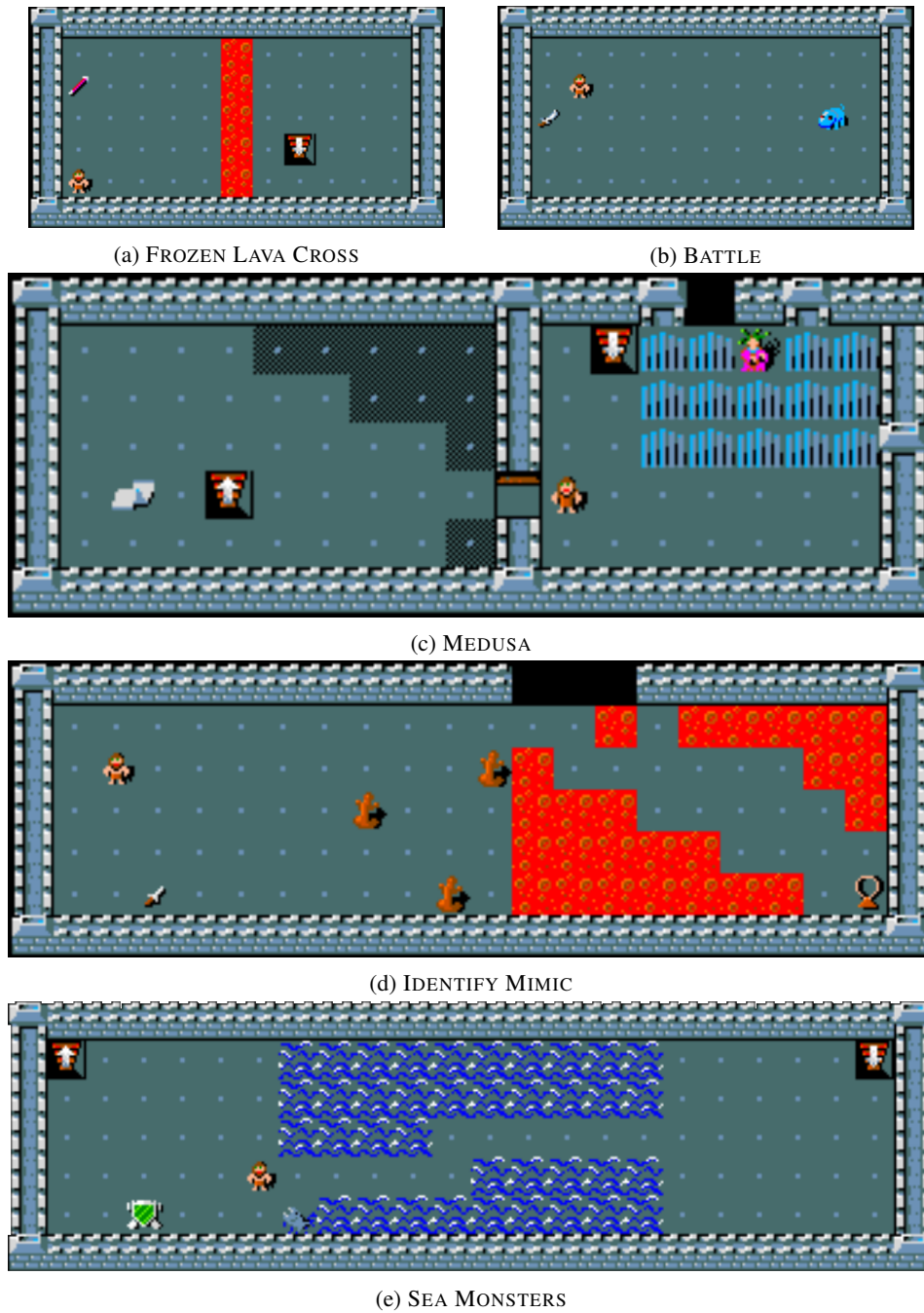
Figure 8: Task environments.
