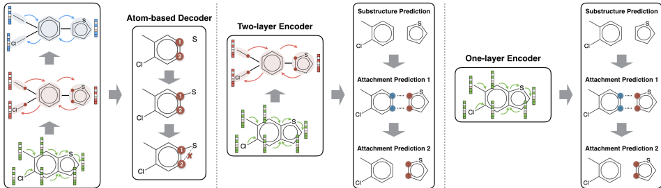
Figure 8: Model Ablations: 1) Atom-based decoder; 2) Two-layer encoder; 3) One-layer encoder.
