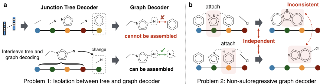
Figure 1: Key limitations of Jin et al. (2019)’s approach: a) Since their tree and graph decoders are isolated, the model can generate invalid junction trees which cannot be assembled into any molecule. This problem can be solved when we interleave the tree and graph decoding steps, allowing the predicted attachments to guide the substructure prediction; b) Their non-autoregressive graph decoder often predicts inconsistent local substructure attachments during training. To this end, we propose an autoregressive decoder that interleaves the prediction of substructures with their attachments.
