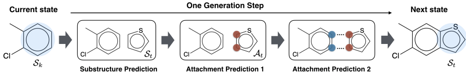
Figure 3: Illustration of hierarchical graph decoding. Suppose the decoder is visiting the substructure S_k . 1) It decides to add a new substructure ( topological prediction ). 2) It predicts that new substructure S_t should be a ring ( substructure prediction ) 3) It predicts how this new ring should be attached to the graph ( attachment prediction ). Finally, the decoder moves to S_t and repeats the process.
