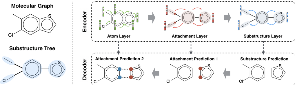
Figure 2: Overview of our approach. Each substructure \mathcal{S}_i is a subgraph of a molecule (e.g., rings). In each step, our decoder adds a new substructure and predicts its attachment to current graph. Our encoder represents each molecule across three levels (atom layer, attachment layer and substructure layer), with each layer capturing relevant information for the corresponding decoding step.
