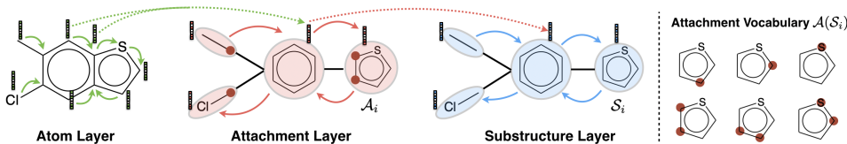
Figure 4: Left: Hierarchical graph encoder. Solid arrows illustrate message passing in each layer. Dashed arrows connect each atom to the substructures it belongs. In the attachment layer, each node \mathcal{A}_i is a particular attachment configuration of substructure \mathcal{S}_i . Right: Attachment vocabulary for a ring. The attaching points in each configuration (highlighted in red) must be consecutive.
