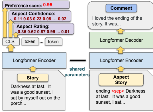
Figure 3: Overview of our model. The encoder (left) predicts the preference score, aspect confidence, and aspect rating. The decoder (right) generates the comment for each aspect.
