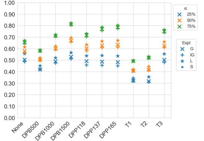
(c) Trustpilot
