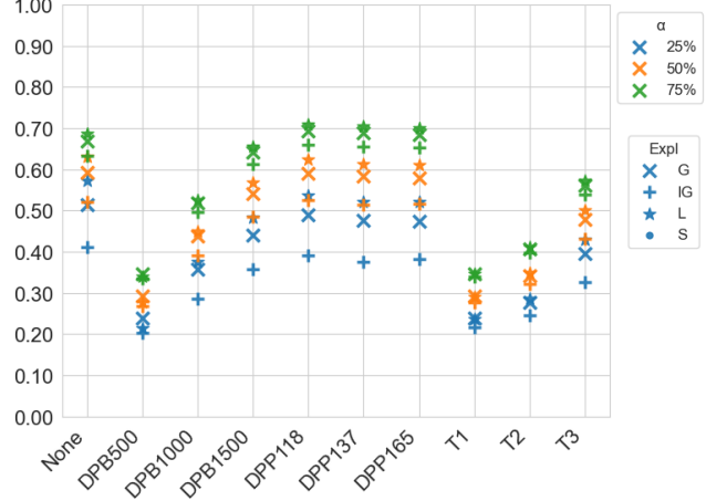
(a) SST2
