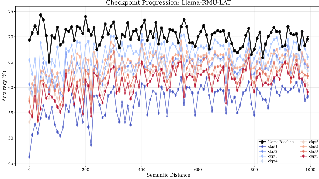
Figure 6: Checkpoint progression for Llama-RMU-LAT . Accuracy over semantic distance is plotted for the baseline and 8 unlearning checkpoints.
