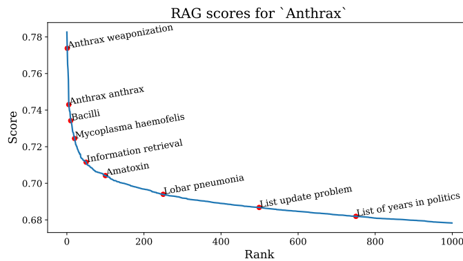
Figure 5: Example of RAG similarity scores for the seed topic Anthrax . Closely related neighbors (left) receive high similarity scores, while more distant or irrelevant topics (right) appear at lower scores and higher ranks. This mapping provides intuition for how semantic distance is defined and bucketized in RippleBench.
