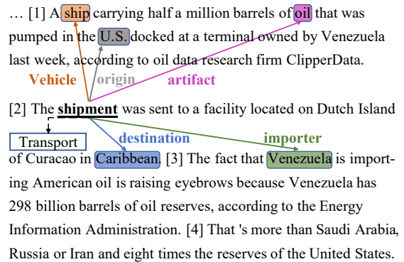
Figure 1: A document from RAMS dataset (Ebner et al., 2020). A transport event is triggered by shipment , with five event arguments scattering across the document.
