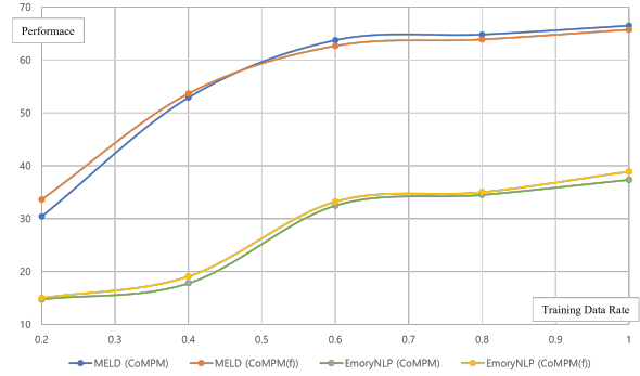
Figure 3: Performance according to the size of training data of CoMPM and EmoryNLP
