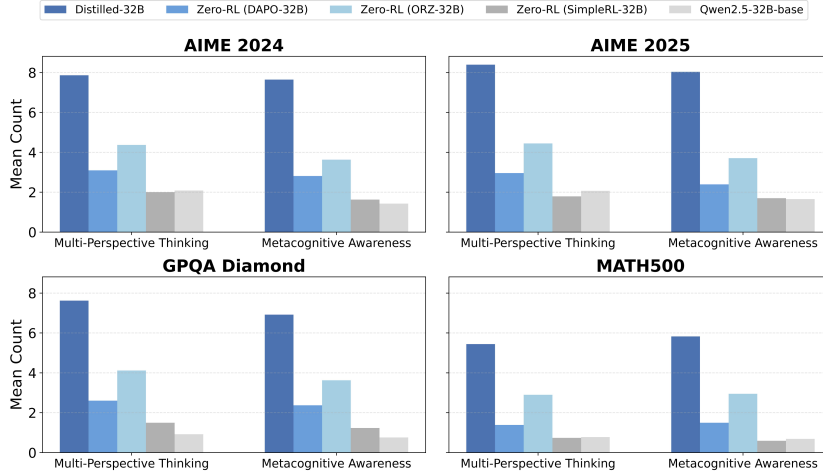
Figure 4: Comparison of the number of advanced cognitive behaviors per response across benchmarks. Additional results are provided in Appendix D.4.
