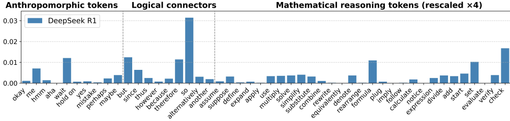
Figure 3: Token usage in DeepSeek R1’s responses to AIME2024 problems across anthropomorphic tokens, logical connectors, and mathematical reasoning tokens.
