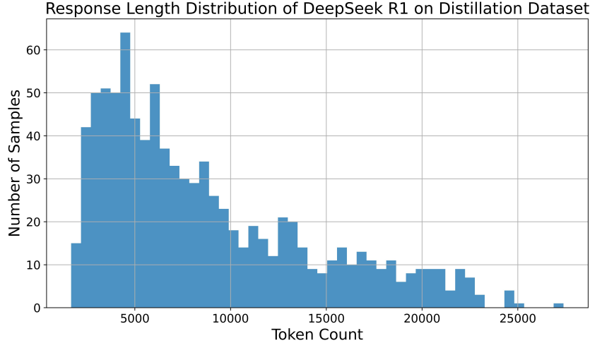
Figure 5: Response length distribution of DeepSeek R1 on 920 distillation problems.
