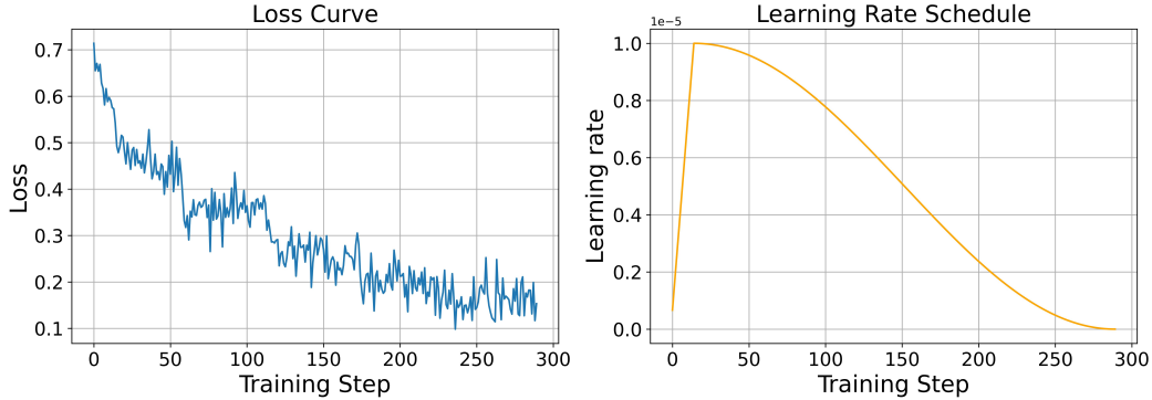
Figure 6: Training curves for our distillation.
