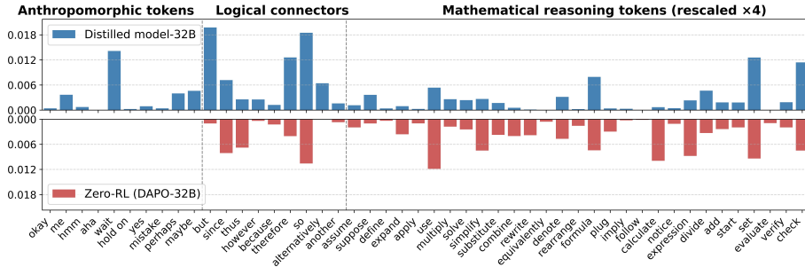
Figure 1: Comparison of token usage between the Distilled and zero-RL models responses to AIME2024 problems across anthropomorphic tokens, logical connectors, and mathematical reasoning tokens. The mathematical reasoning tokens are rescaled by a factor of 4 for better visibility.
