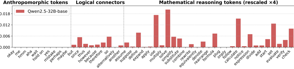
Figure 2: Token usage in Qwen2.5-32B-base’s responses to AIME2024 problems across anthropomorphic tokens, logical connectors, and mathematical reasoning tokens.
