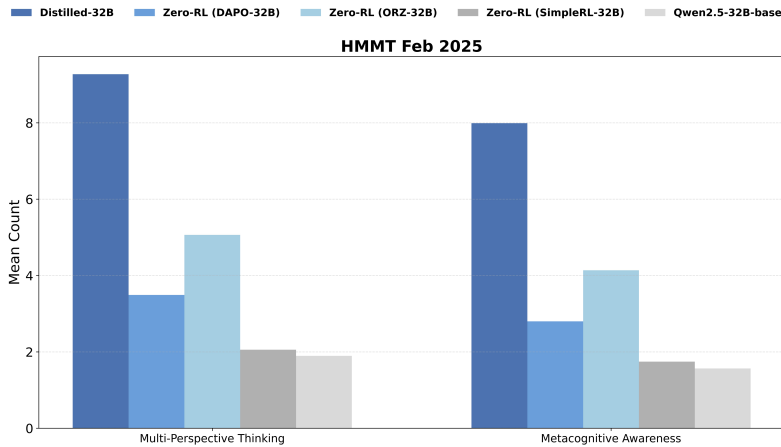
Figure 7: Comparison of the number of advanced cognitive behaviors per response on HMMT Feb 2025.
