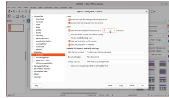
(f) Change the time to 3 minutes: agent.type(230, "3", overwrite=True)
