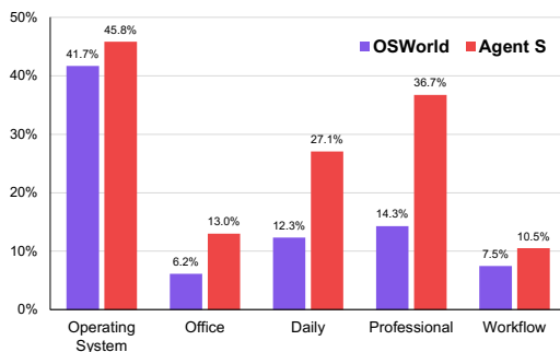
Figure 2: Agent S vs. OSWorld Agent results across five broad computer task categories.
