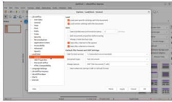
(e) Click on the General sub-option: agent.click(208, 1, left)
