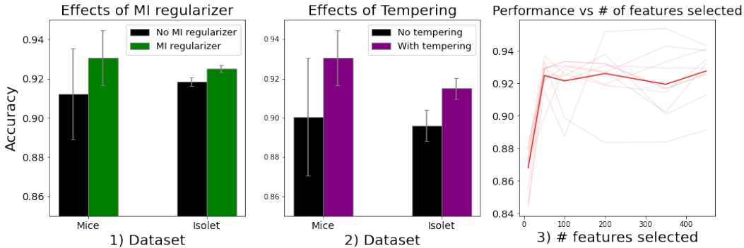
Figure 2: (1) and (2) show ablation studies on the effect of MI regularization and tempering the number of features. R3: Both ablation studies have the same number (50) of selected features on all datasets. (3) shows the task accuracy as a function of the number of features selected on the activity dataset. The dark line shows the average of ten random hyperparameter trials, shown with light hue, demonstrating that task performance can be near-optimal even with a small subset of features.
