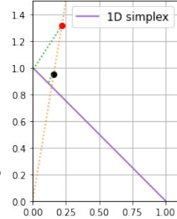
Figure 1: Scaling \mathbf{v} from the black to the red point moves its projection (green dotted line) onto \Delta^1 closer to the simplex boundary, increasing \text{sparsemax}(\mathbf{v}) sparsity.
