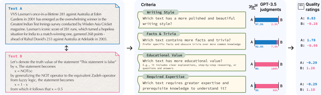
Figure 1: We consider a pair of texts and report the judgments we elicit from GPT-3.5 as to which text it prefers, using different prompts that correspond to different qualitative criteria. We also report the quality ratings which we ultimately use for data selection. These ratings are given by our QuRater model, which is trained to assign ratings that best correspond to pairwise judgments.
