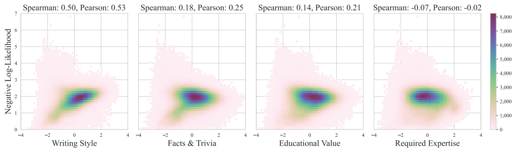
Figure 6: Correlations of quality ratings and negative log-likelihood scores by Llama-2-7B(Touvron et al., 2023b) over 1M training sequences. The negative log-likelihoods are averaged over the number of tokens, and are the logarithm of the perplexity score of a single sequence. We observe that perplexity scores are not good approximations for any quality criteria.
