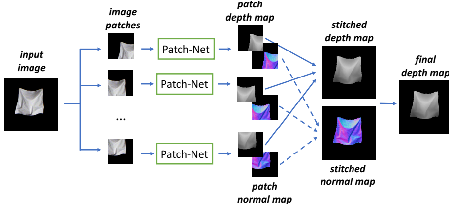
Figure 1: Patch-based 3D reconstruction from a single image. The input image is split into overlapping patches and prediction of depth and normal maps per patch is performed using Patch-Net. Patch depth maps are stitched by translating each depth map along the camera viewing direction in order to minimize the relative depth difference at overlapping regions and averaging the depth at overlapping regions. Patch normal maps are stitched by normalizing and averaging the predictions at overlapping regions. Both the stitched depth and normal maps are refined using bilateral filtering at the patch boundaries. The final depth map is estimated after normals integration with a depth scale factor inferred by the stitched depth map.
