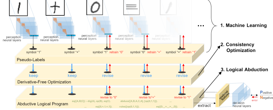
Figure 5: The structure of our ABL implementation.
