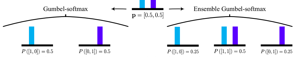
Figure 2: A visualized comparison between Gumbel-Softmax (left) and ensemble Gumbel-Softmax (right, M = 2 ). For a probability vector \mathbf{p} = [0.5, 0.5] , Gumbel-Softmax solely pertains to sample only two binary codes with the same probability, i.e. , P([1, 0]) = P([0, 1]) = 0.5 . In contrast, our ensemble Gumbel-Softmax is capable of sampling more diversified binary codes, i.e. , [1, 0] , [1, 1] and [0, 1] . Furthermore, the probabilities of sampling these binary codes are logical. Typically, it is conceptually intuitive that the probability of sampling [1, 1] is larger than the probabilities of sampling the others since the probabilities in \mathbf{p} = [0.5, 0.5] are equal to each other.
