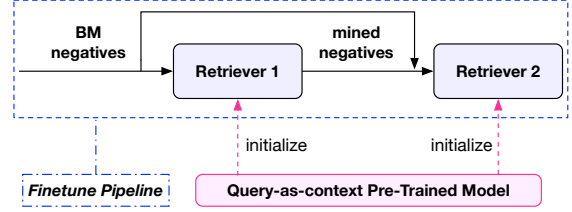
Figure 3: Illustration of the fine-tuning pipeline. The query-as-context pre-trained model is used to initialize the dual-encoder retrievers.
