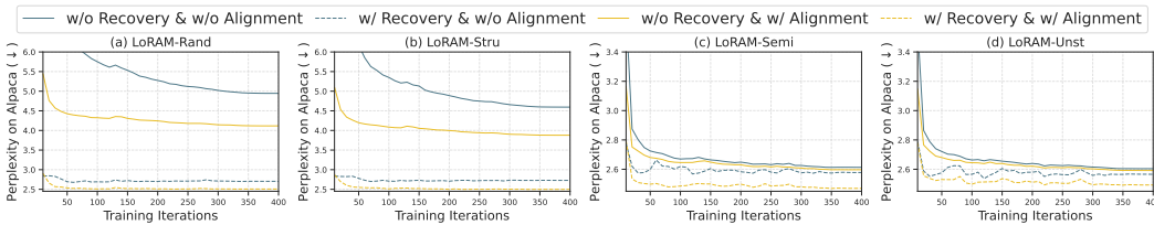
Figure 6: Necessity of Recovery & Alignment across different pruning strategies on LLaMA-2-13B.
