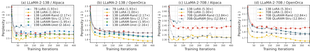
Figure 4: The test perplexity of training LLaMA-2-13B & LLaMA-2-70B on OpenOrca.
