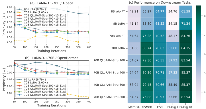
Figure 5: The test perplexity & downstream performance of training LLaMA-3.1-70B on OpenHermes.
