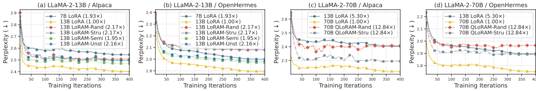
Figure 3: The test perplexity of training LLaMA-2-13B & LLaMA-2-70B on OpenHermes.
