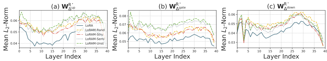
Figure 11: Average L_2 norms of low-rank matrices in the MLP layers of LLaMA-2-70B.
